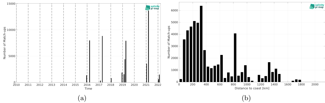
Figure 2: Number of match-ups between TSG (CSIC-UTM) and SMAP SSS L2 v5.3 - 40 km (RSS) SSS as a function of time (a) and as function of the distance to coast (b) over the Roaring Forties and Furious Fifties Pi-MEP region and for the full satellite product period.
