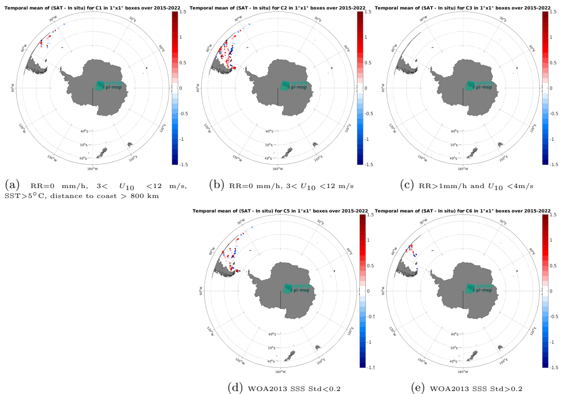
Figure 14: Temporal mean gridded over spatial boxes of size 1^\circ \times 1^\circ of \Delta SSS (SMAP SSS L2 v5.3 - 40 km (RSS) - TSG (CSIC-UTM)) for 5 different subdatasets corresponding to:RR=0 mm/h, 3 < U_{10} < 12 m/s, SST>5°C, distance to coast > 800 km (a), RR=0 mm/h, 3 < U_{10} < 12 m/s (b), RR>1mm/h and U_{10} < 4 m/s (c), WOA2013 SSS Std<0.2 (d), WOA2013 SSS Std>0.2 (e).
