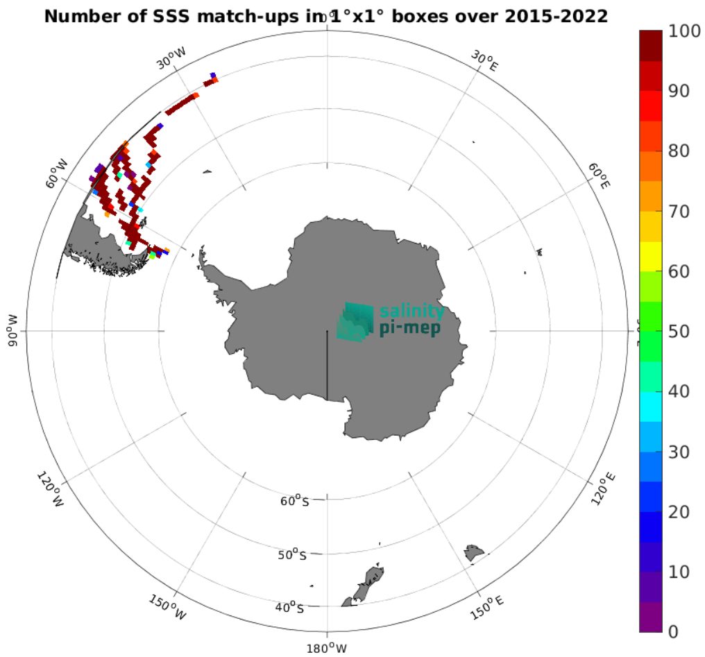
Figure 5: Number of SSS match-ups between TSG (CSIC-UTM) SSS and the SMAP SSS L2 v5.3 - 40 km (RSS) SSS product for the Roaring Forties and Furious Fifties Pi-MEP region over 1^\circ \times 1^\circ boxes and for the full satellite product period.
