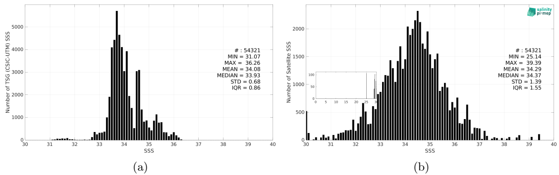
Figure 3: Histograms of SSS from TSG (CSIC-UTM) (a) and SMAP SSS L2 v5.3 - 40 km (RSS) (b) considering all match-up pairs per bins of 0.1 over the Roaring Forties and Furious Fifties Pi-MEP region and for the full satellite product period.
