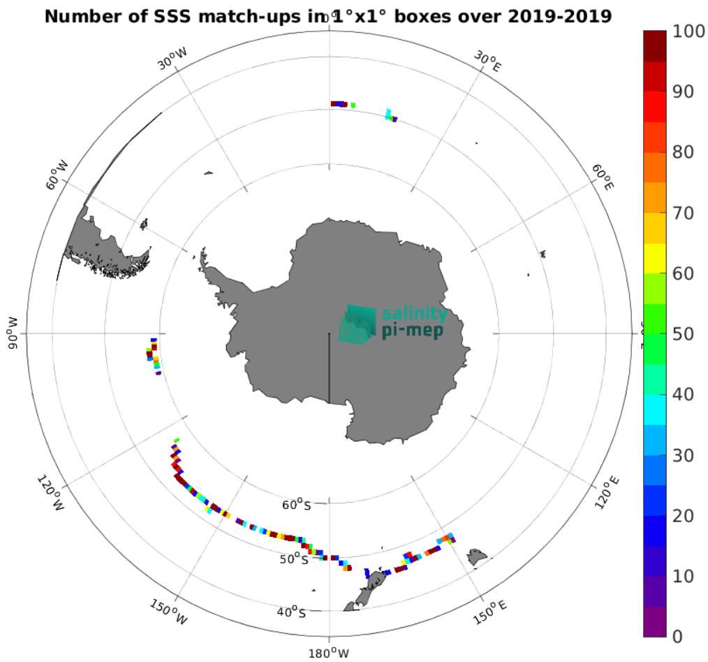
Figure 5: Number of SSS match-ups between Sairdrone SSS and the SMAP SSS L2 v5.3 - 40 km (RSS) SSS product for the Roaring Forties and Furious Fifties Pi-MEP region over 1^{\circ} \times 1^{\circ} boxes and for the full satellite product period.
