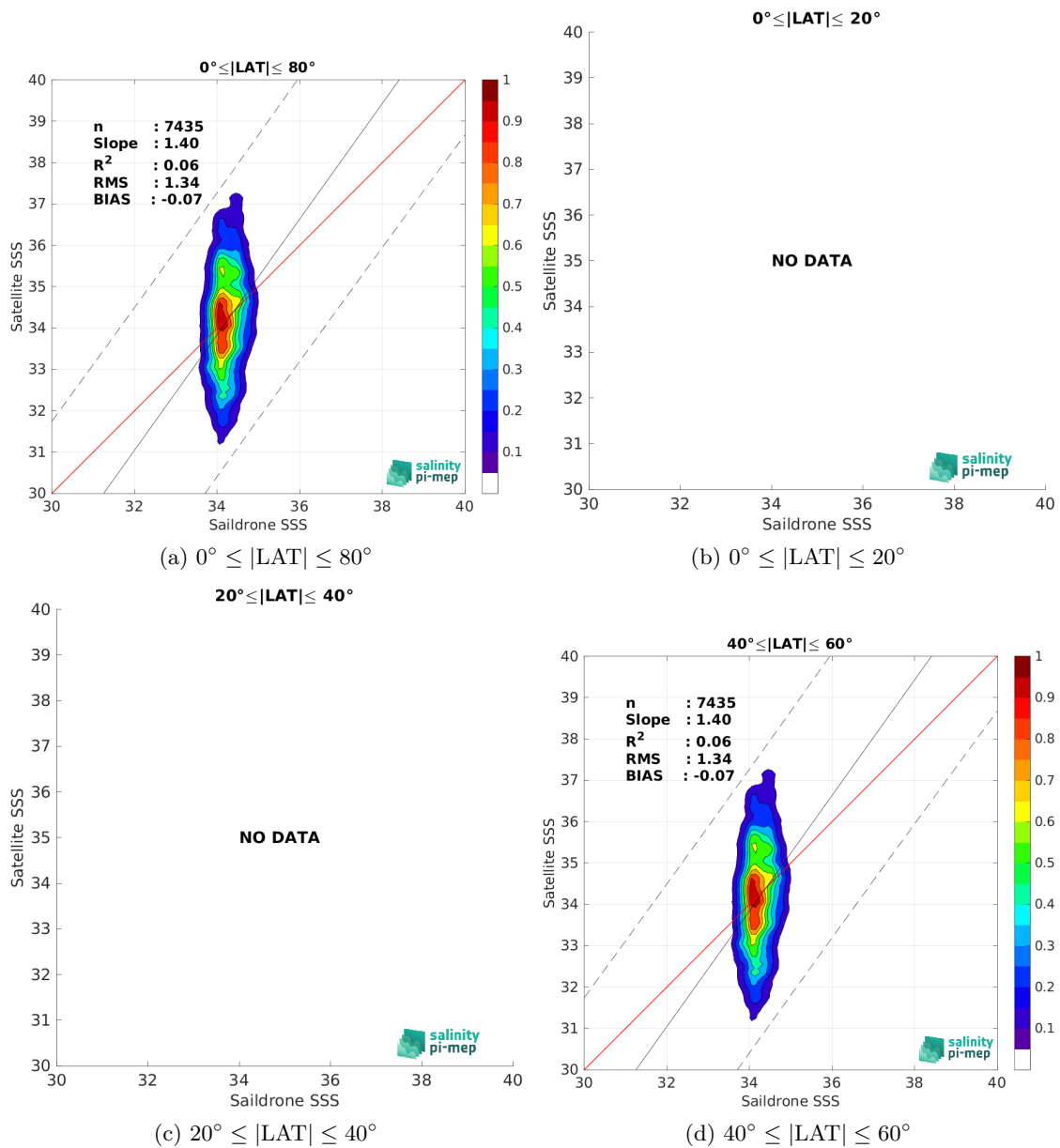
Figure 10: Contour maps of the concentration of SMAP SSS L2 v5.3 - 40 km (RSS) SSS (y-axis) versus Saldrone SSS (x-axis) at match-up pairs for different latitude bands. For each plot, the red line shows x=y . The black thin and dashed lines indicate a linear fit through the data cloud and the \pm 95\% confidence levels, respectively. The number match-up pairs n , the slope and R^2 coefficient of the linear fit, the root mean square (RMS) and the mean bias between satellite and in situ data are indicated for each latitude band in each plots.
