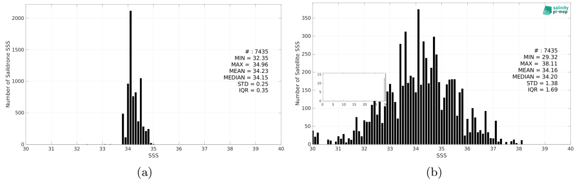
Figure 3: Histograms of SSS from Saildrone (a) and SMAP SSS L2 v5.3 - 40 km (RSS) (b) considering all match-up pairs per bins of 0.1 over the Roaring Forties and Furious Fifties Pi-MEP region and for the full satellite product period.
