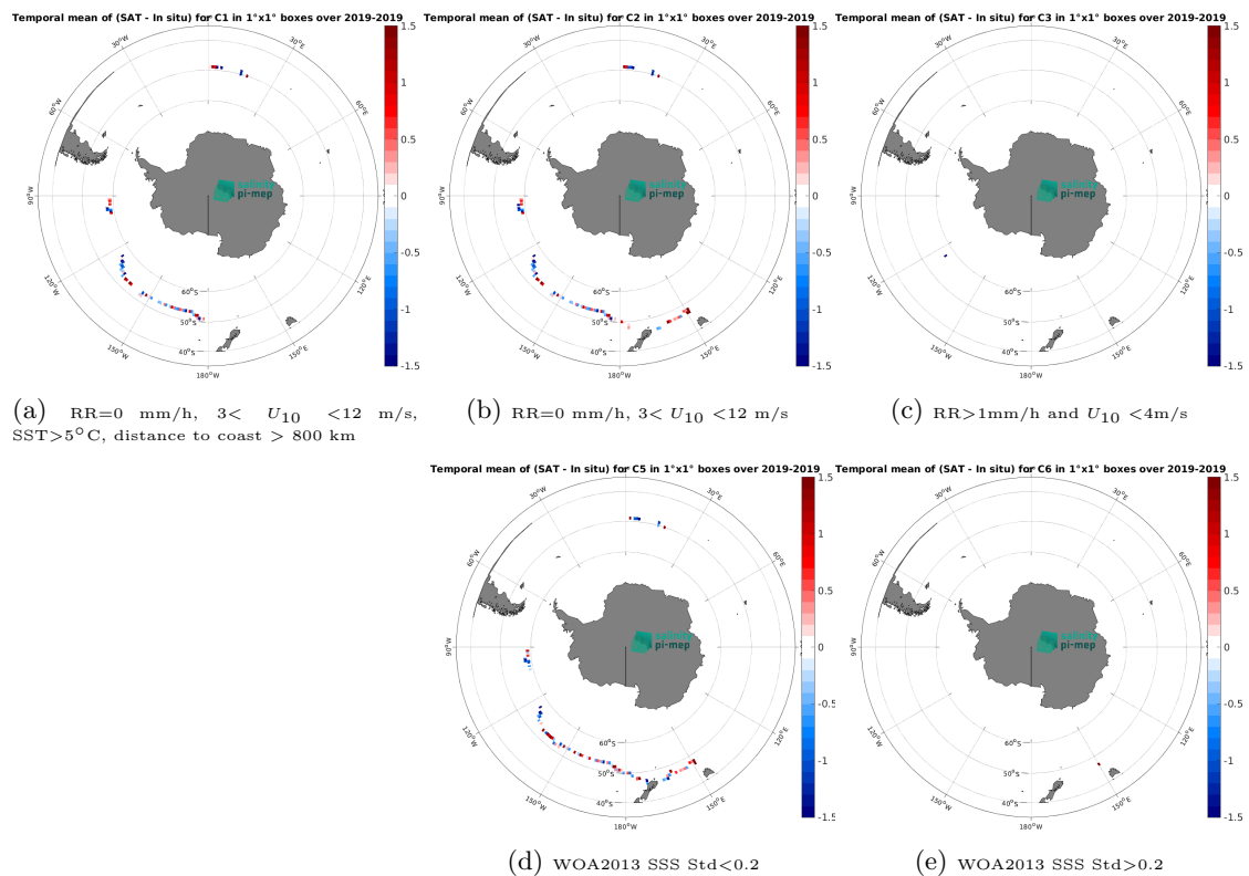
Figure 14: Temporal mean gridded over spatial boxes of size 1^\circ \times 1^\circ of \Delta SSS (SMAP SSS L2 v5.3 - 40 km (RSS) - Sailydrone) for 5 different subdatasets corresponding to:RR=0 mm/h, 3 < U_{10} < 12 m/s, SST>5°C, distance to coast > 800 km (a), RR=0 mm/h, 3 < U_{10} < 12 m/s (b), RR>1mm/h and U_{10} < 4 m/s (c), WOA2013 SSS Std<0.2 (d), WOA2013 SSS Std>0.2 (e).
