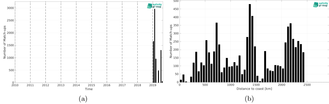
Figure 2: Number of match-ups between Saildrone and SMAP SSS L2 v5.3 - 40 km (RSS) SSS as a function of time (a) and as function of the distance to coast (b) over the Roaring Forties and Furious Fifties Pi-MEP region and for the full satellite product period.
