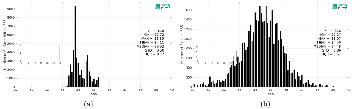
Figure 3: Histograms of SSS from Surface drifters (a) and SMAP SSS L2 v5.3 - 40 km (RSS) (b) considering all match-up pairs per bins of 0.1 over the Roaring Forties and Furious Fifties Pi-MEP region and for the full satellite product period.
