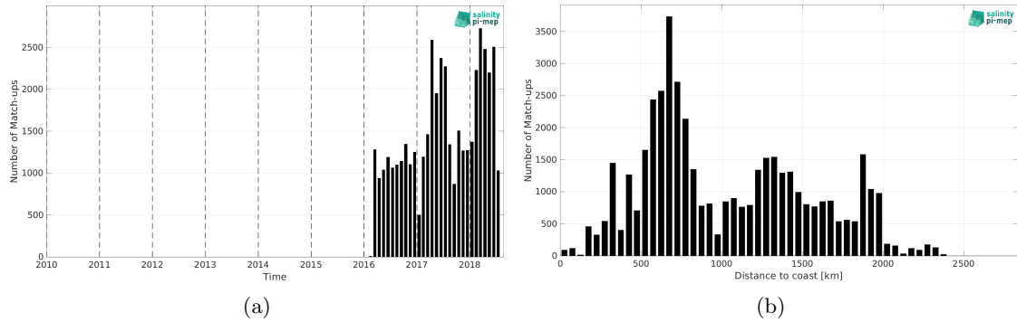
Figure 2: Number of match-ups between Surface drifters and SMAP SSS L2 v5.3 - 40 km (RSS) SSS as a function of time (a) and as function of the distance to coast (b) over the Roaring Forties and Furious Fifties Pi-MEP region and for the full satellite product period.
