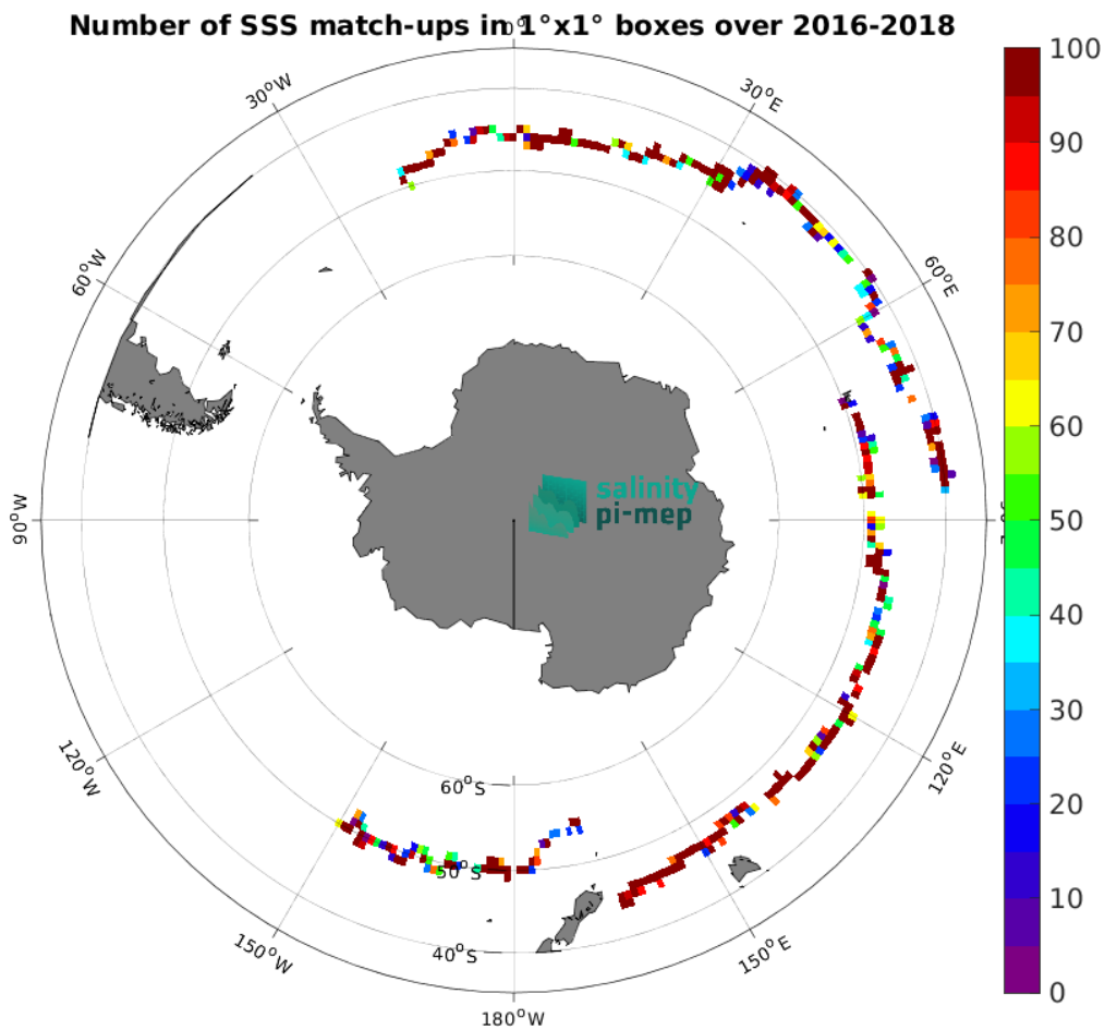
Figure 4: Number of SSS match-ups between Surface drifters SSS and the SMAP SSS L2 v5.3 - 40 km (RSS) SSS product for the Roaring Forties and Furious Fifties Pi-MEP region over 1^\circ \times 1^\circ boxes and for the full satellite product period.
