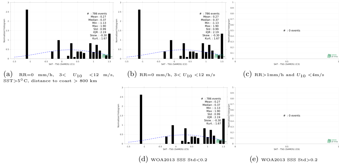
Figure 13: Normalized histogram of \Delta SSS (SMAP SSS L2 v5 - 40 km (RSS) - TSG (SAMOS)) for 5 different subdatasets corresponding to: RR=0 mm/h, 3 < U_{10} < 12 m/s, SST > 5°C, distance to coast > 800 km (a), RR=0 mm/h, 3 < U_{10} < 12 m/s (b), RR > 1mm/h and U_{10} < 4 m/s (c), WOA2013 SSS Std < 0.2 (d), WOA2013 SSS Std > 0.2 (e).
