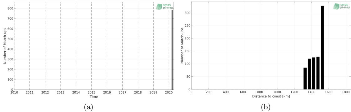
Figure 1: Number of match-ups between TSG (SAMOS) and SMAP SSS L2 v5 - 40 km (RSS) SSS as a function of time (a) and as function of the distance to coast (b) over the Roaring Forties and Furious Fifties Pi-MEP region and for the full satellite product period.
