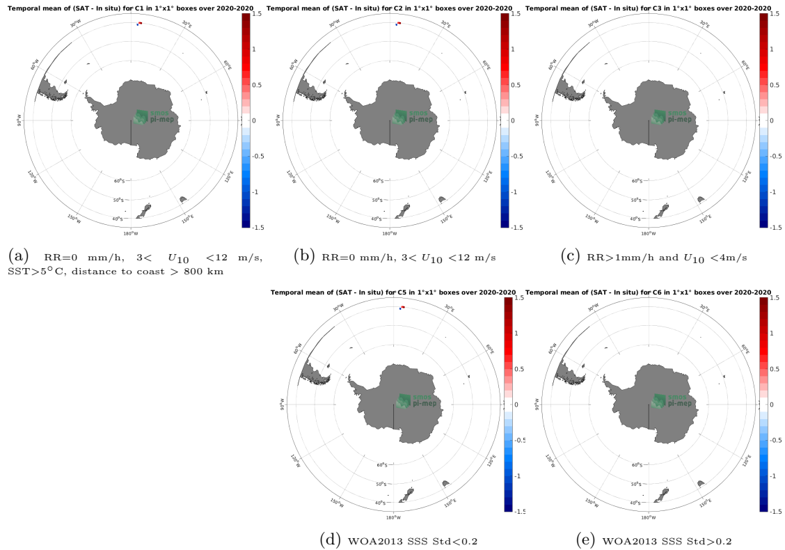
Figure 12: Temporal mean gridded over spatial boxes of size 1^{\circ}\times 1^{\circ} of \Delta\text{SSS} (SMAP SSS L2 v5 - 40 km (RSS) - TSG (SAMOS)) for 5 different subdatasets corresponding to:RR=0 mm/h, 3 < U_{10} < 12 m/s, SST >5^{\circ}\text{C} , distance to coast > 800 km (a), RR=0 mm/h, 3 < U_{10} < 12 m/s (b), RR >1 mm/h and U_{10} < 4 m/s (c), WOA2013 SSS Std <0.2 (d), WOA2013 SSS Std >0.2 (e).
