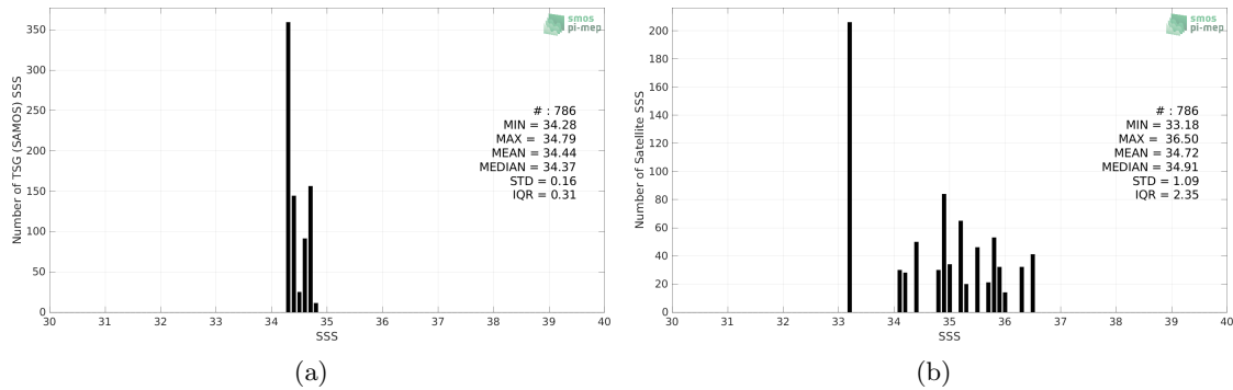
Figure 2: Histograms of SSS from TSG (SAMOS) (a) and SMAP SSS L2 v5 - 40 km (RSS) (b) considering all match-up pairs per bins of 0.1 over the Roaring Forties and Furious Fifties Pi-MEP region and for the full satellite product period.
