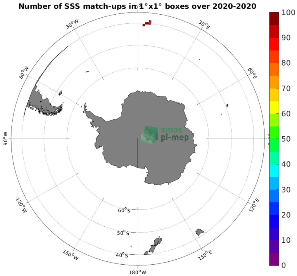
Figure 4: Number of SSS match-ups between TSG (SAMOS) SSS and the SMAP SSS L2 v5 - 40 km (RSS) SSS product for the Roaring Forties and Furious Fifties Pi-MEP region over 1^\circ \times 1^\circ boxes and for the full satellite product period.
