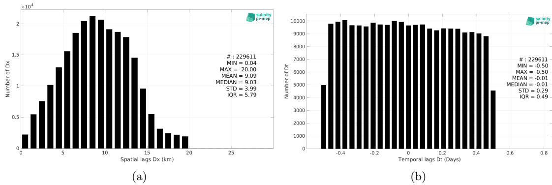
Figure 5: Histograms of the spatial (a) and temporal (b) lags between the location/time of the TSG (LEGOS-DM) measurement and the date of the corresponding SMAP SSS L2 v5 - 40 km (RSS) SSS pixel.
