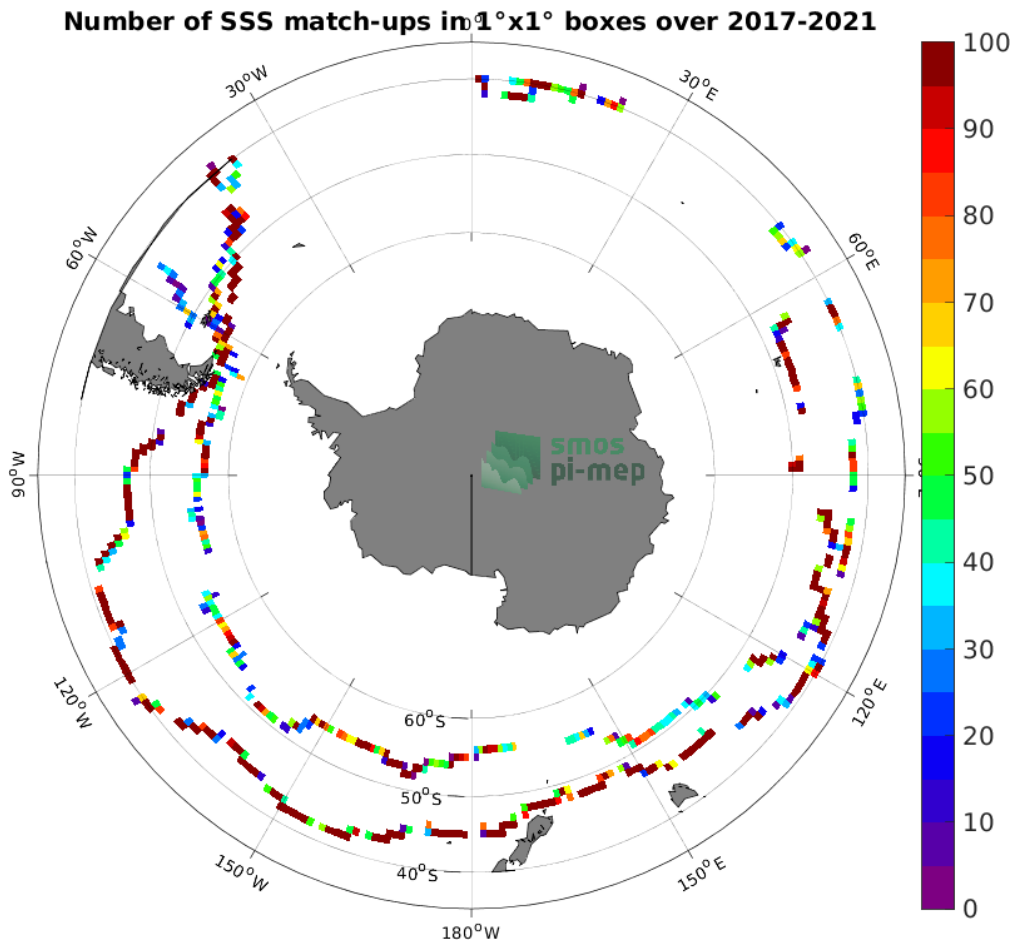
Figure 4: Number of SSS match-ups between TSG (GOSUD-Sailing-ship) SSS and the SMAP SSS L2 v5 - 40 km (RSS) SSS product for the Roaring Forties and Furious Fifties Pi-MEP region over 1^\circ \times 1^\circ boxes and for the full satellite product period.
