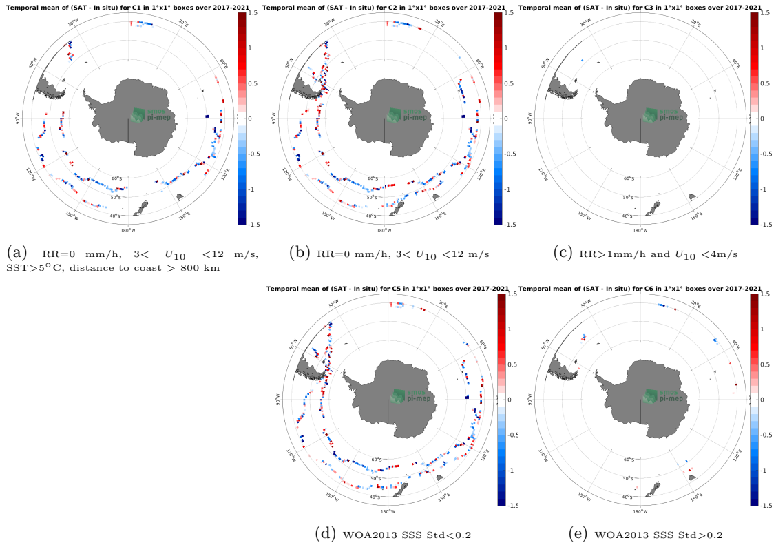
Figure 12: Temporal mean gridded over spatial boxes of size 1°x1° of \Delta SSS (SMAP SSS L2 v5 - 40 km (RSS) - TSG (GOSUD-Sailing-ship)) for 5 different subdatasets corresponding to:RR=0 mm/h, 3 < U_{10} < 12 m/s, SST>5°C, distance to coast > 800 km (a), RR=0 mm/h, 3 < U_{10} < 12 m/s (b), RR>1mm/h and U_{10} < 4 m/s (c), WOA2013 SSS Std<0.2 (d), WOA2013 SSS Std>0.2 (e).
