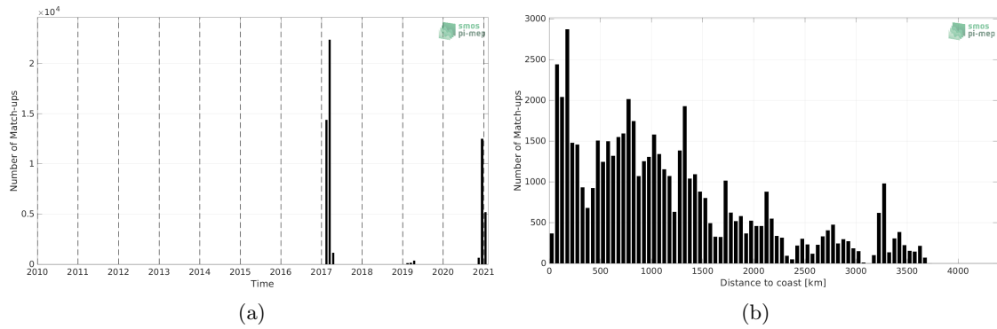
Figure 1: Number of match-ups between TSG (GOSUD-Sailing-ship) and SMAP SSS L2 v5 - 40 km (RSS) SSS as a function of time (a) and as function of the distance to coast (b) over the Roaring Forties and Furious Fifties Pi-MEP region and for the full satellite product period.
