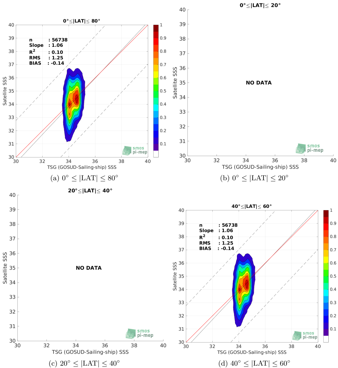
Figure 9: Contour maps of the concentration of SMAP SSS L2 v5 - 40 km (RSS) SSS (y-axis) versus TSG (GOSUD-Sailing-ship) SSS (x-axis) at match-up pairs for different latitude bands. For each plot, the red line shows x=y . The black thin and dashed lines indicate a linear fit through the data cloud and the \pm 95\% confidence levels, respectively. The number match-up pairs n , the slope and R^2 coefficient of the linear fit, the root mean square (RMS) and the mean bias between satellite and in situ data are indicated for each latitude band in each plots.
