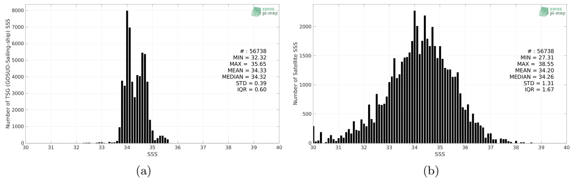
Figure 2: Histograms of SSS from TSG (GOSUD-Sailing-ship) (a) and SMAP SSS L2 v5 - 40 km (RSS) (b) considering all match-up pairs per bins of 0.1 over the Roaring Forties and Furious Fifties Pi-MEP region and for the full satellite product period.
