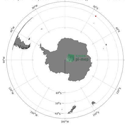
(e) MEAN( \Delta SSS) (Satellite - TSG (GOSUD-Research-vessel))
