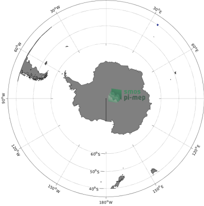
(c) MEAN(TSG (GOSUD-Research-vessel) SSS)
