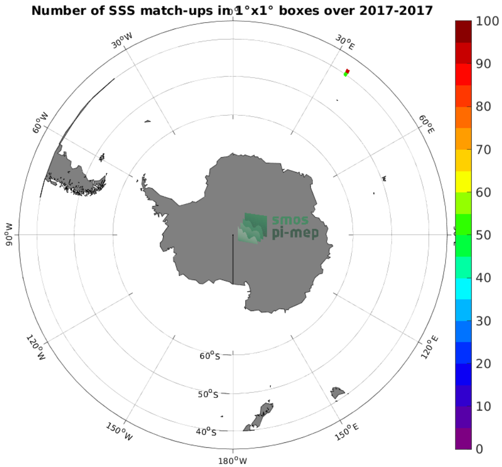
Figure 4: Number of SSS match-ups between TSG (GOSUD-Research-vessel) SSS and the SMAP SSS L2 v5 - 40 km (RSS) SSS product for the Roaring Forties and Furious Fifties Pi-MEP region over 1^\circ \times 1^\circ boxes and for the full satellite product period.
