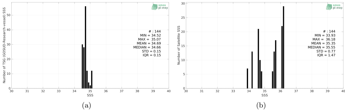
Figure 2: Histograms of SSS from TSG (GOSUD-Research-vessel) (a) and SMAP SSS L2 v5 - 40 km (RSS) (b) considering all match-up pairs per bins of 0.1 over the Roaring Forties and Furious Fifties Pi-MEP region and for the full satellite product period.
