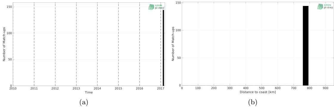
Figure 1: Number of match-ups between TSG (GOSUD-Research-vessel) and SMAP SSS L2 v5 - 40 km (RSS) SSS as a function of time (a) and as function of the distance to coast (b) over the Roaring Forties and Furious Fifties Pi-MEP region and for the full satellite product period.
