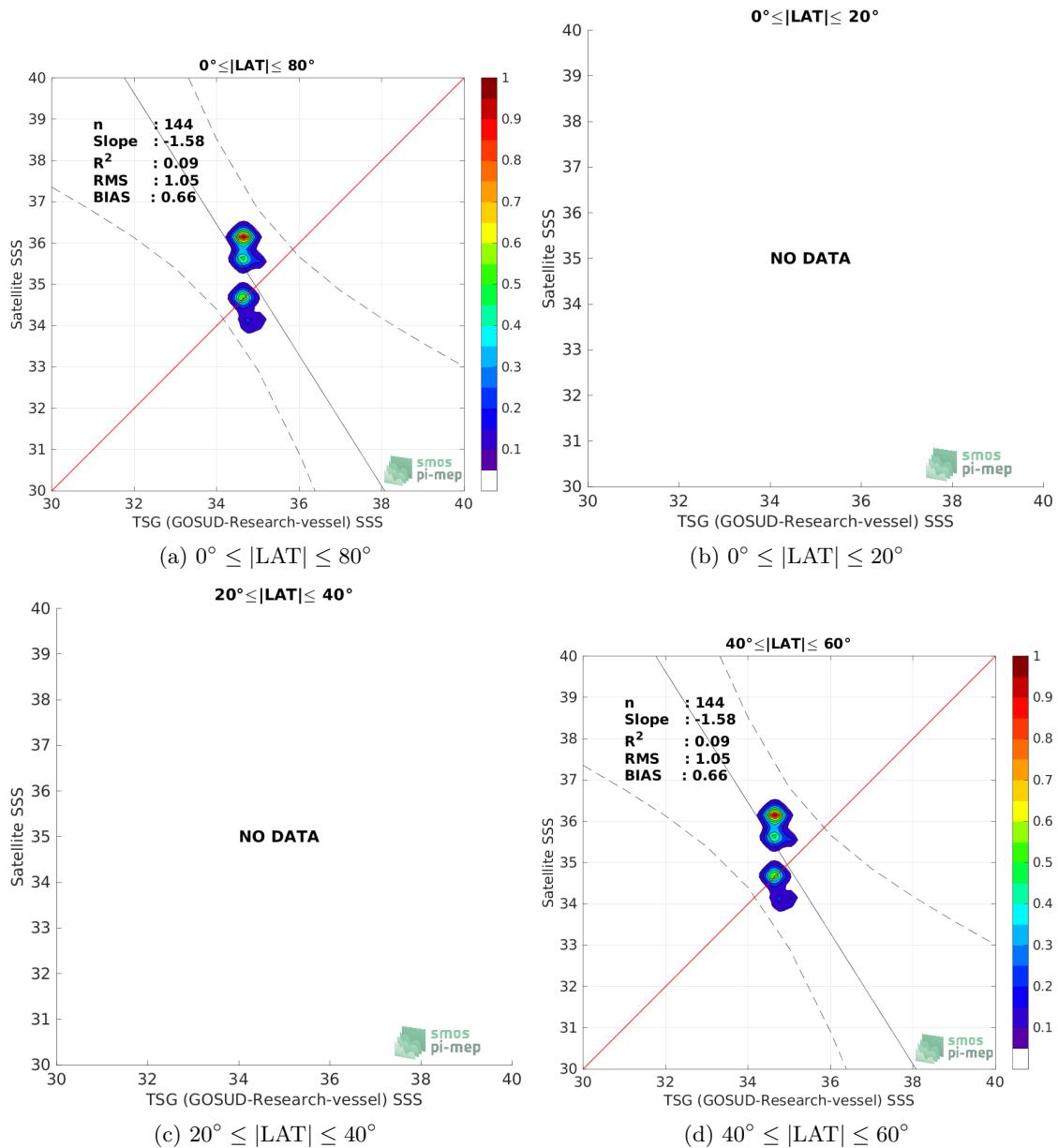
Figure 9: Contour maps of the concentration of SMAP SSS L2 v5 - 40 km (RSS) SSS (y-axis) versus TSG (GOSUD-Research-vessel) SSS (x-axis) at match-up pairs for different latitude bands. For each plot, the red line shows x=y . The black thin and dashed lines indicate a linear fit through the data cloud and the \pm 95\% confidence levels, respectively. The number match-up pairs n , the slope and R^2 coefficient of the linear fit, the root mean square (RMS) and the mean bias between satellite and in situ data are indicated for each latitude band in each plot.
