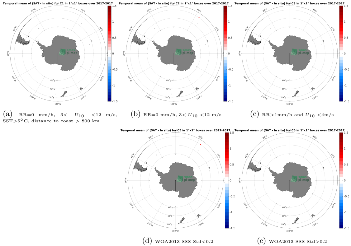
Figure 12: Temporal mean gridded over spatial boxes of size 1^\circ \times 1^\circ of \Delta\text{SSS} (SMAP SSS L2 v5 - 40 km (RSS) - TSG (GOSUD-Research-vessel)) for 5 different subdatasets corresponding to: RR=0 mm/h, 3 < U_{10} < 12 m/s, SST > 5^\circ\text{C} , distance to coast > 800 km (a), RR=0 mm/h, 3 < U_{10} < 12 m/s (b), RR > 1 mm/h and U_{10} < 4 m/s (c), WOA2013 SSS Std < 0.2 (d), WOA2013 SSS Std > 0.2 (e).
