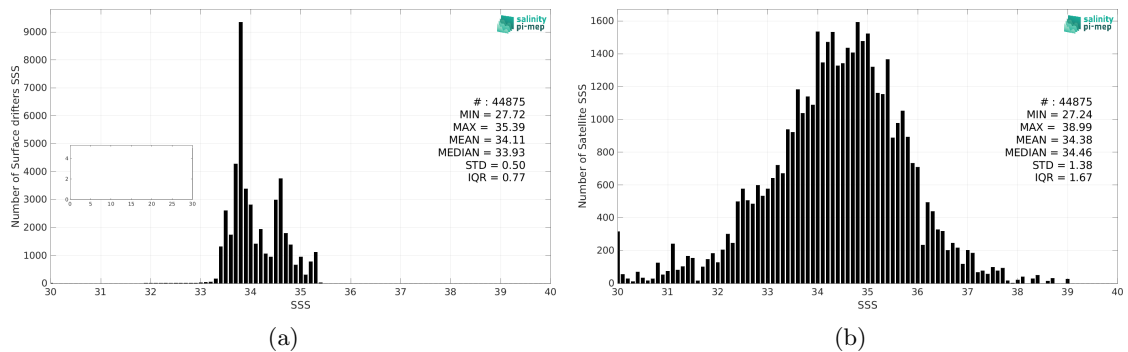
Figure 2: Histograms of SSS from Surface drifters (a) and SMAP SSS L2 v5 - 40 km (RSS) (b) considering all match-up pairs per bins of 0.1 over the Roaring Forties and Furious Fifties Pi-MEP region and for the full satellite product period.
