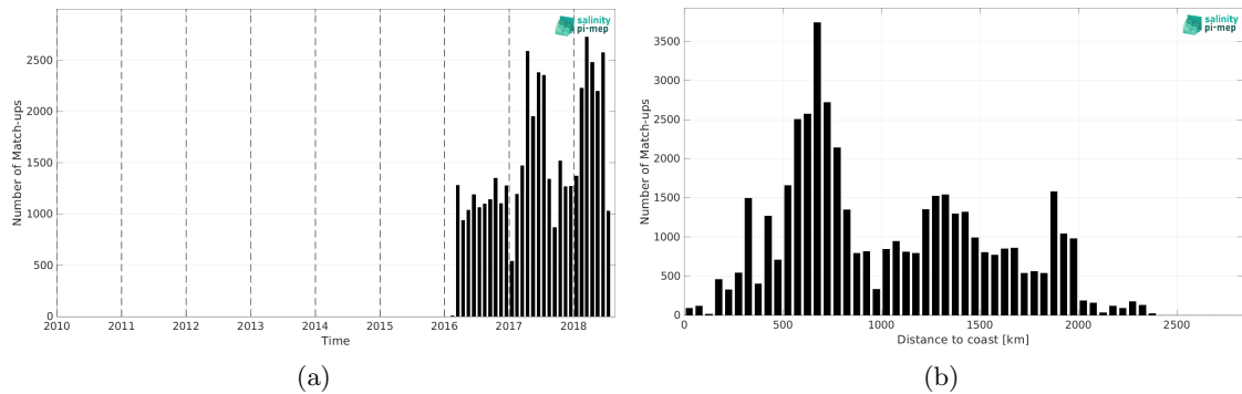
Figure 1: Number of match-ups between Surface drifters and SMAP SSS L2 v5 - 40 km (RSS) SSS as a function of time (a) and as function of the distance to coast (b) over the Roaring Forties and Furious Fifties Pi-MEP region and for the full satellite product period.
