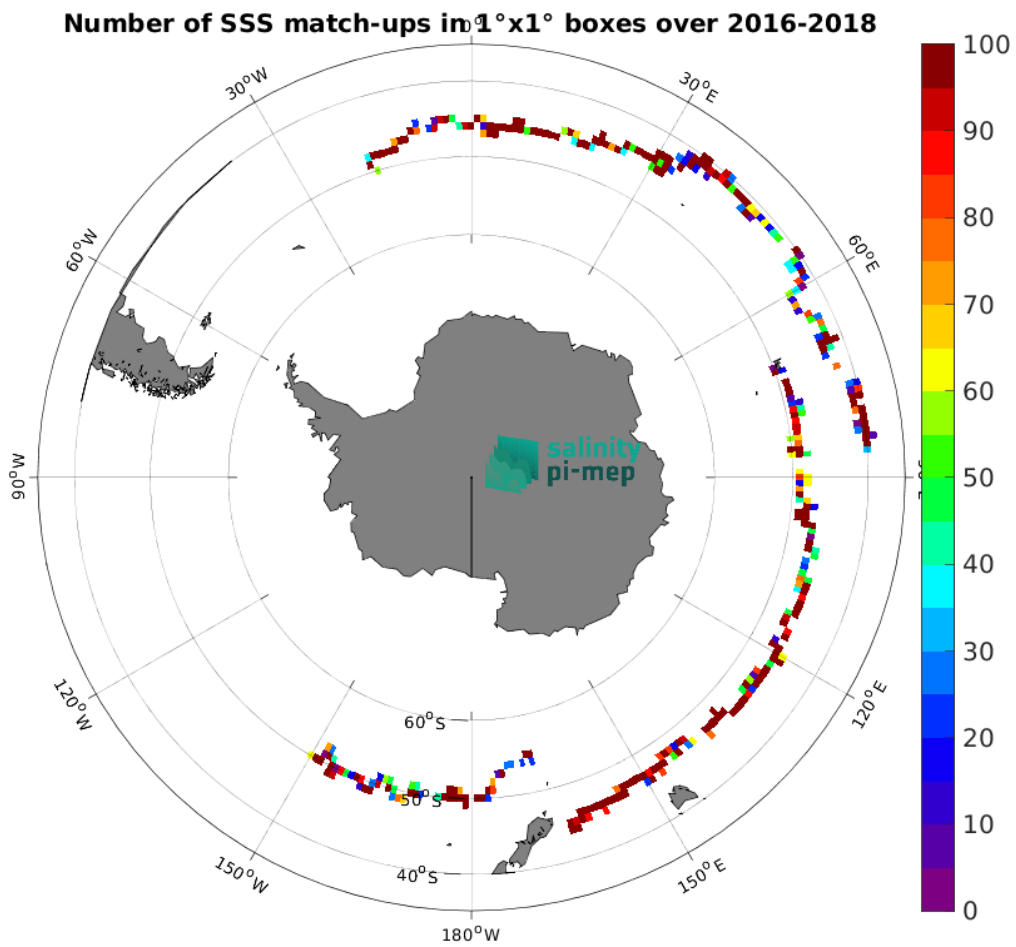
Figure 3: Number of SSS match-ups between Surface drifters SSS and the SMAP SSS L2 v5 - 40 km (RSS) SSS product for the Roaring Forties and Furious Fifties Pi-MEP region over 1^\circ \times 1^\circ boxes and for the full satellite product period.
