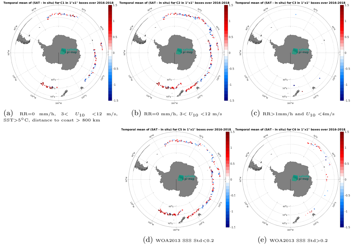
Figure 11: Temporal mean gridded over spatial boxes of size 1^{\circ}\times 1^{\circ} of \Delta\text{SSS} (SMAP SSS L2 v5 - 40 km (RSS) - Surface drifters) for 5 different subdatasets corresponding to:RR=0 mm/h, 3 < U_{10} < 12 m/s, SST >5^{\circ}\text{C} , distance to coast > 800 km (a), RR=0 mm/h, 3 < U_{10} < 12 m/s (b), RR >1 mm/h and U_{10} < 4 m/s (c), WOA2013 SSS Std <0.2 (d), WOA2013 SSS Std >0.2 (e).
