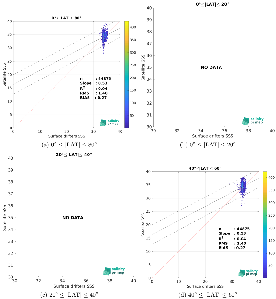
Figure 8: Contour maps of the concentration of SMAP SSS L2 v5 - 40 km (RSS) SSS (y-axis) versus Surface drifters SSS (x-axis) at match-up pairs for different latitude bands. For each plot, the red line shows x=y . The black thin and dashed lines indicate a linear fit through the data cloud and the \pm 95\% confidence levels, respectively. The number match-up pairs n , the slope and R^2 coefficient of the linear fit, the root mean square (RMS) and the mean bias between satellite and in situ data are indicated for each latitude band in each plots.
