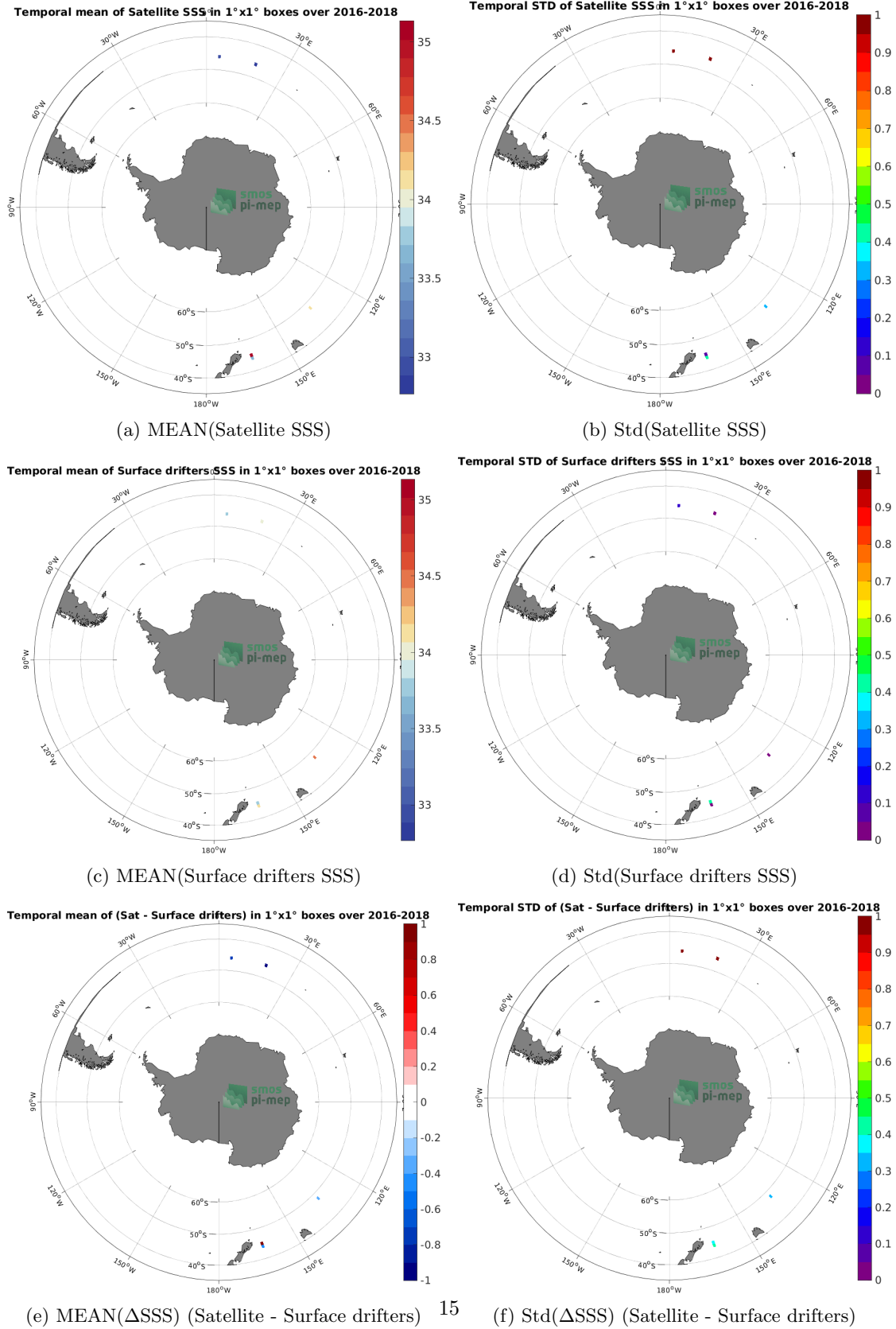
Figure 5: Temporal mean (left) and Std (right) of SSS from SMAP SSS L2 v5 - 40 km (RSS) (top), Surface drifters (middle), and of \Delta SSS (Satellite - Surface drifters). Only match-up pairs are used to generate these maps.
