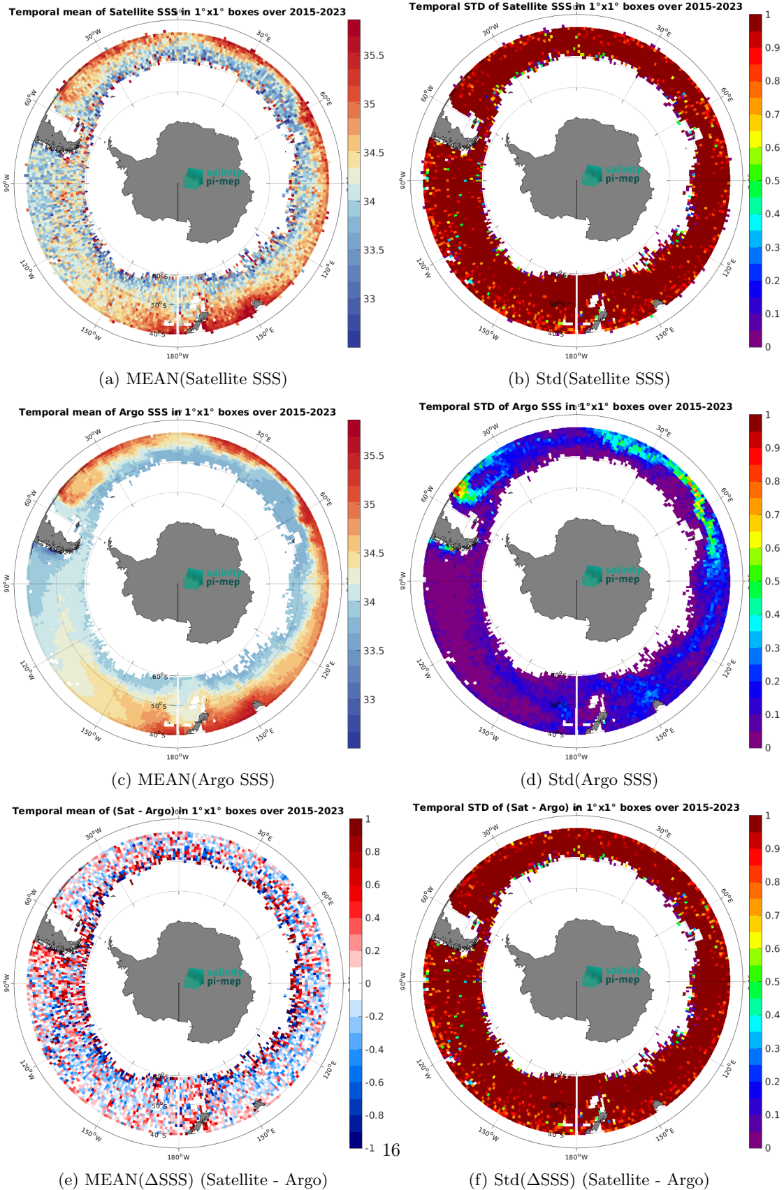
Figure 6: Temporal mean (left) and Std (right) of SSS from SMAP SSS L2 v5 - 40 km (RSS) (top), Argo (middle), and of \Delta SSS (Satellite - Argo). Only match-up pairs are used to generate these maps.
