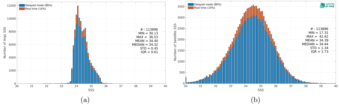
Figure 2: Histograms of SSS from Argo (a) and SMAP SSS L2 v5 - 40 km (RSS) (b) considering all match-up pairs per bins of 0.1 over the Roaring Forties and Furious Fifties Pi-MEP region and for the full satellite product period.
