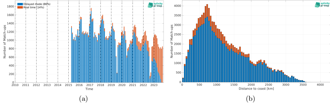
Figure 1: Number of match-ups between Argo and SMAP SSS L2 v5 - 40 km (RSS) SSS as a function of time (a) and as function of the distance to coast (b) over the Roaring Forties and Furious Fifties Pi-MEP region and for the full satellite product period.
