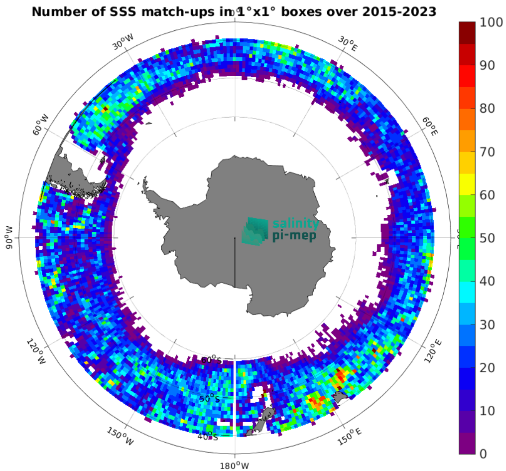
Figure 4: Number of SSS match-ups between Argo SSS and the SMAP SSS L2 v5 - 40 km (RSS) SSS product for the Roaring Forties and Furious Fifties Pi-MEP region over 1^\circ \times 1^\circ boxes and for the full satellite product period.
