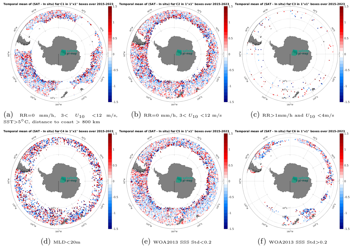
Figure 12: Temporal mean gridded over spatial boxes of size 1^{\circ}\times 1^{\circ} of \Delta\text{SSS} (SMAP SSS L2 v5 - 40 km (RSS) - Argo) for 6 different subdatasets corresponding to:RR=0 mm/h, 3 < U_{10} < 12 m/s, SST >5^{\circ}\text{C} , distance to coast > 800 km (a), RR=0 mm/h, 3 < U_{10} < 12 m/s (b), RR >1 mm/h and U_{10} < 4 m/s (c),MLD <20 m (d),WOA2013 SSS Std <0.2 (e),WOA2013 SSS Std >0.2 (f).
