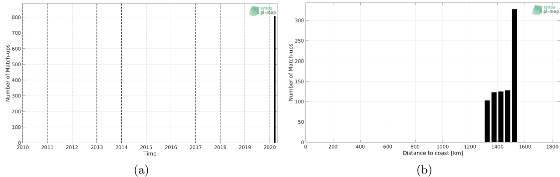
Figure 1: Number of match-ups between TSG (SAMOS) and SMAP SSS L2 v4 (RSS) SSS as a function of time (a) and as function of the distance to coast (b) over the Roaring Forties and Furious Fifties Pi-MEP region and for the full satellite product period.
