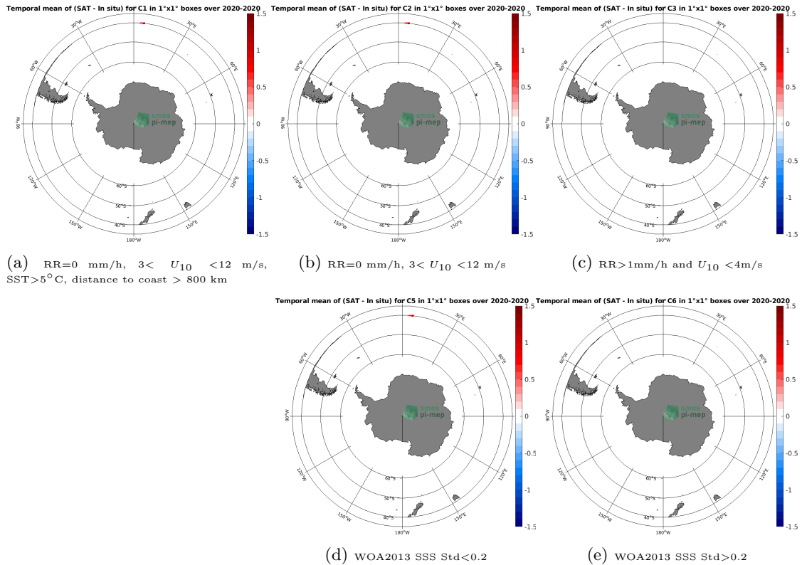
Figure 12: Temporal mean gridded over spatial boxes of size 1^{\circ}\times 1^{\circ} of \Delta\text{SSS} (SMAP SSS L2 v4 (RSS) - TSG (SAMOS)) for 5 different subdatasets corresponding to:RR=0 mm/h, 3 < U_{10} < 12 m/s, SST >5^{\circ}\text{C} , distance to coast > 800 km (a), RR=0 mm/h, 3 < U_{10} < 12 m/s (b), RR >1\text{mm/h} and U_{10} < 4\text{m/s} (c), WOA2013 SSS Std <0.2 (d), WOA2013 SSS Std >0.2 (e).
