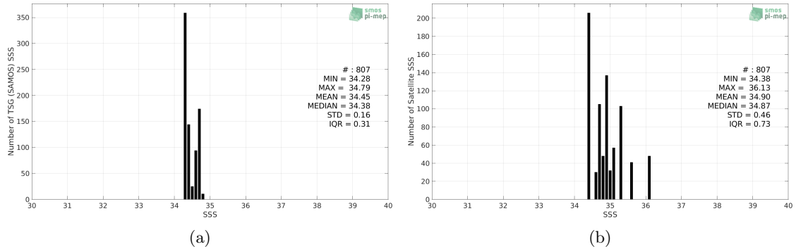
Figure 2: Histograms of SSS from TSG (SAMOS) (a) and SMAP SSS L2 v4 (RSS) (b) considering all match-up pairs per bins of 0.1 over the Roaring Forties and Furious Fifties Pi-MEP region and for the full satellite product period.
