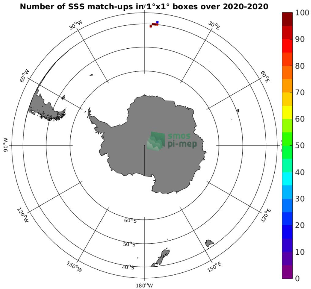
Figure 4: Number of SSS match-ups between TSG (SAMOS) SSS and the SMAP SSS L2 v4 (RSS) SSS product for the Roaring Forties and Furious Fifties Pi-MEP region over 1°x1° boxes and for the full satellite product period.
