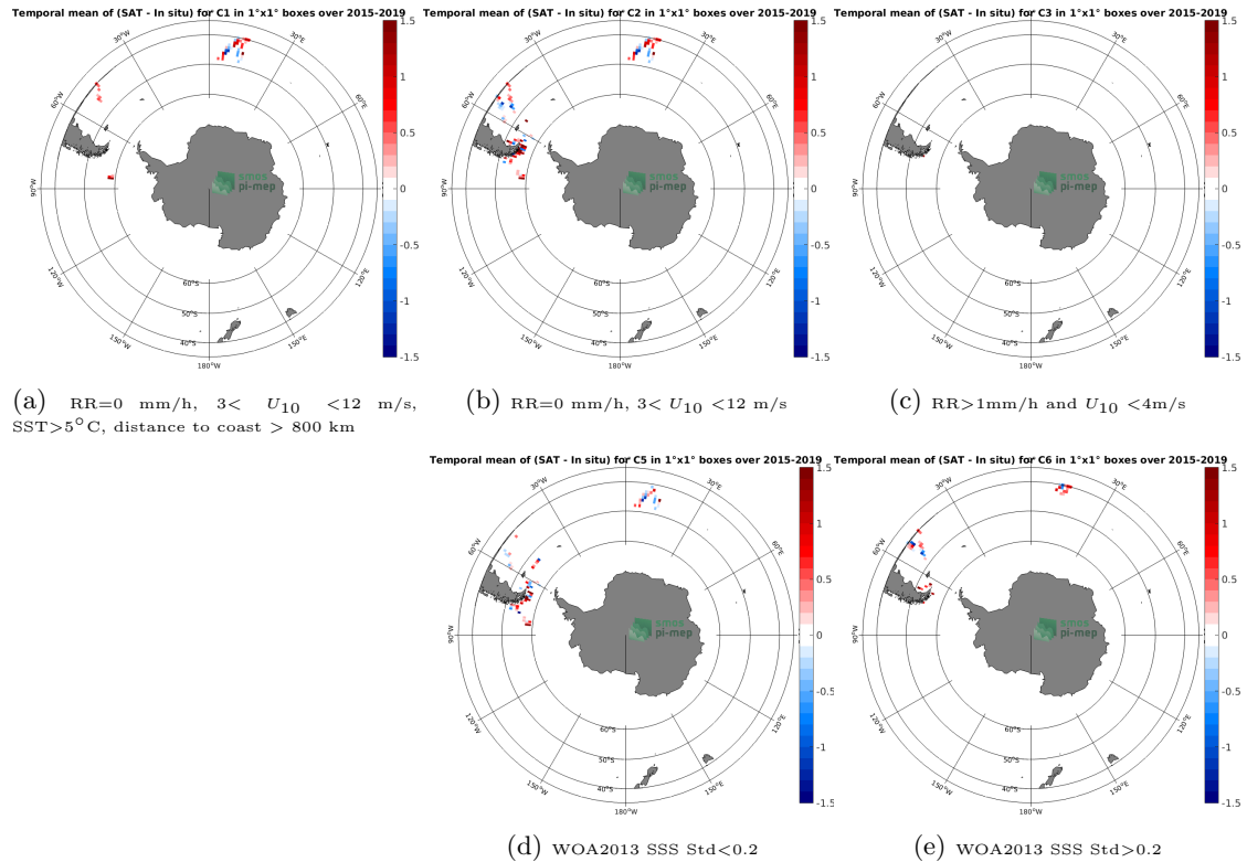
Figure 12: Temporal mean gridded over spatial boxes of size 1^{\circ}\times 1^{\circ} of \Delta\text{SSS} (SMAP SSS L2 v4 (RSS) - TSG (Polarstern)) for 5 different subdatasets corresponding to: \text{RR}=0 mm/h, 3 < U_{10} < 12 m/s, \text{SST}>5^{\circ}\text{C} , distance to coast > 800 km (a), \text{RR}=0 mm/h, 3 < U_{10} < 12 m/s (b), \text{RR}>1\text{mm/h} and U_{10} < 4\text{m/s} (c), WOA2013 SSS Std < 0.2 (d), WOA2013 SSS Std > 0.2 (e).
