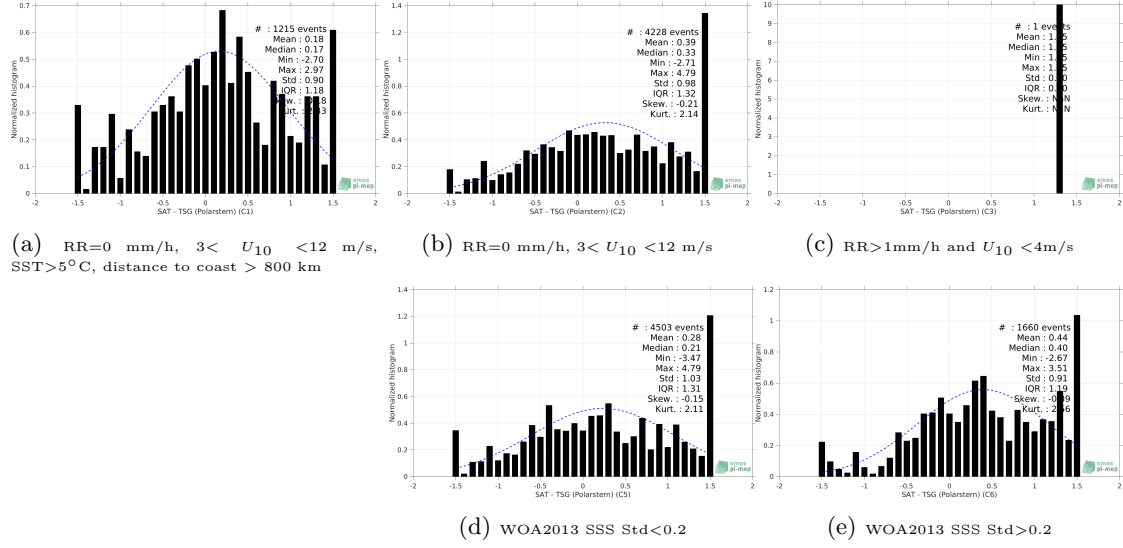
Figure 13: Normalized histogram of \Delta\text{SSS} (SMAP SSS L2 v4 (RSS) - TSG (Polarstern)) for 5 different subdatasets corresponding to: RR=0 mm/h, 3 < U_{10} < 12 m/s, SST>5°C, distance to coast > 800 km (a), RR=0 mm/h, 3 < U_{10} < 12 m/s (b), RR>1mm/h and U_{10} < 4 m/s (c), WOA2013 SSS Std<0.2 (d), WOA2013 SSS Std>0.2 (e).
