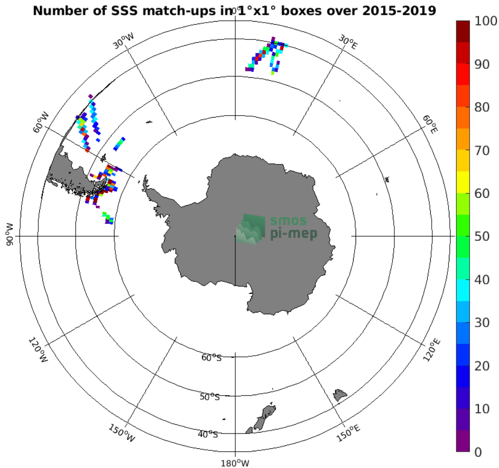
Figure 4: Number of SSS match-ups between TSG (Polarstern) SSS and the SMAP SSS L2 v4 (RSS) SSS product for the Roaring Forties and Furious Fifties Pi-MEP region over 1^\circ \times 1^\circ boxes and for the full satellite product period.
