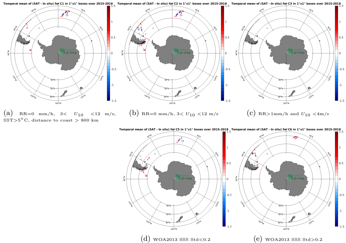
Figure 12: Temporal mean gridded over spatial boxes of size 1^{\circ}\times 1^{\circ} of \Delta\text{SSS} (SMAP SSS L2 v4 (RSS) - TSG (Polarstern)) for 5 different subdatasets corresponding to:RR=0 mm/h, 3 < U_{10} < 12 m/s, SST >5^{\circ}\text{C} , distance to coast > 800 km (a), RR=0 mm/h, 3 < U_{10} < 12 m/s (b), RR >1 mm/h and U_{10} < 4 m/s (c), WOA2013 SSS Std <0.2 (d), WOA2013 SSS Std >0.2 (e).
