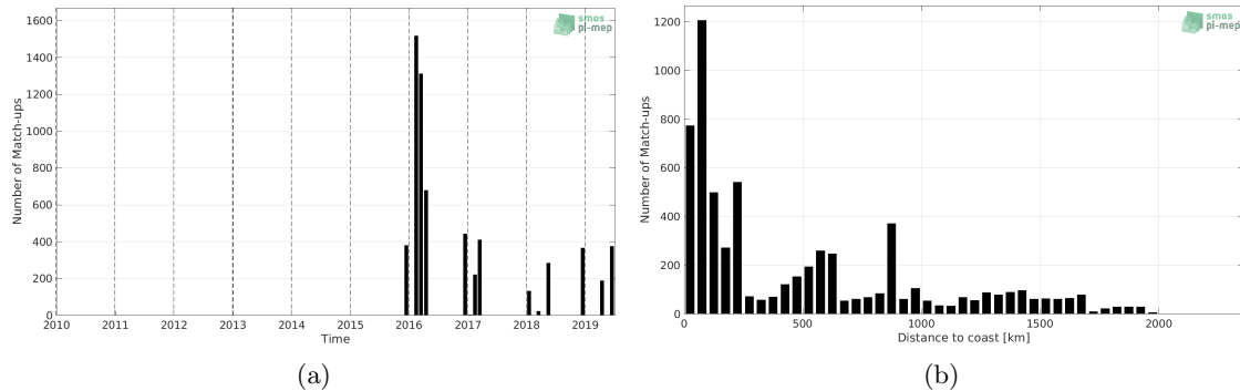
Figure 1: Number of match-ups between TSG (Polarstern) and SMAP SSS L2 v4 (RSS) SSS as a function of time (a) and as function of the distance to coast (b) over the Roaring Forties and Furious Fifties Pi-MEP region and for the full satellite product period.
