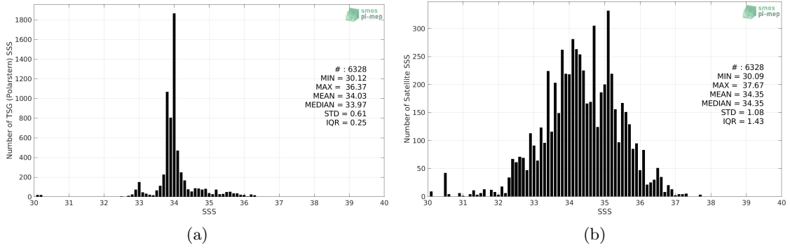
Figure 2: Histograms of SSS from TSG (Polarstern) (a) and SMAP SSS L2 v4 (RSS) (b) considering all match-up pairs per bins of 0.1 over the Roaring Forties and Furious Fifties Pi-MEP region and for the full satellite product period.
