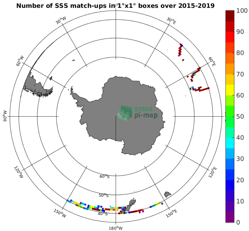
Figure 4: Number of SSS match-ups between TSG-LEGOS-DM SSS and the SMAP-L2-RSS-V4 SSS product for the Roaring Forties and Furious Fifties Pi-MEP region over 1^\circ \times 1^\circ boxes and for the full satellite product period.
