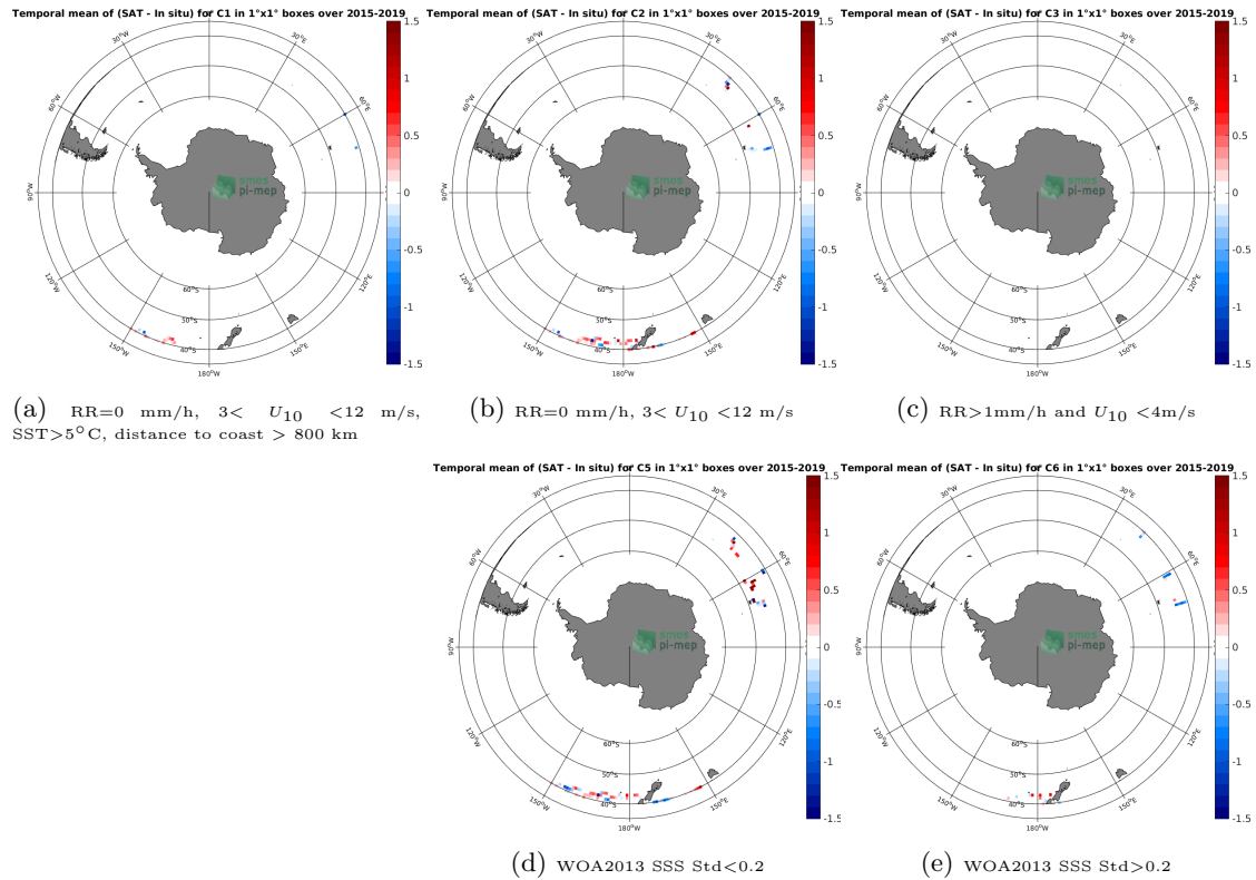
Figure 12: Temporal mean gridded over spatial boxes of size 1^{\circ}\times 1^{\circ} of \Delta\text{SSS} (SMAP-L2-RSS-V4 - TSG-LEGOS-DM) for 5 different subdatasets corresponding to: \text{RR}=0 mm/h, 3 < U_{10} < 12 m/s, \text{SST}>5^{\circ}\text{C} , distance to coast > 800 km (a), \text{RR}=0 mm/h, 3 < U_{10} < 12 m/s (b), \text{RR}>1 mm/h and U_{10} < 4 m/s (c), WOA2013 SSS Std <0.2 (d), WOA2013 SSS Std >0.2 (e).
