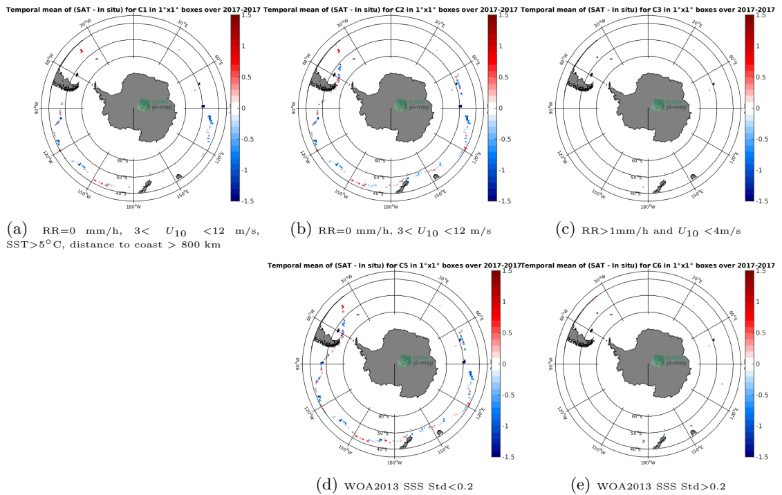
Figure 12: Temporal mean gridded over spatial boxes of size 1^\circ \times 1^\circ of \Delta SSS (SMAP-L2-RSS-V4 - TSG-GOSUD-Sailing-ship) for 5 different subdatasets corresponding to: RR=0 mm/h, 3 < U_{10} < 12 m/s, SST > 5°C, distance to coast > 800 km (a), RR=0 mm/h, 3 < U_{10} < 12 m/s (b), RR > 1mm/h and U_{10} < 4 m/s (c), WOA2013 SSS Std < 0.2 (d), WOA2013 SSS Std > 0.2 (e).
