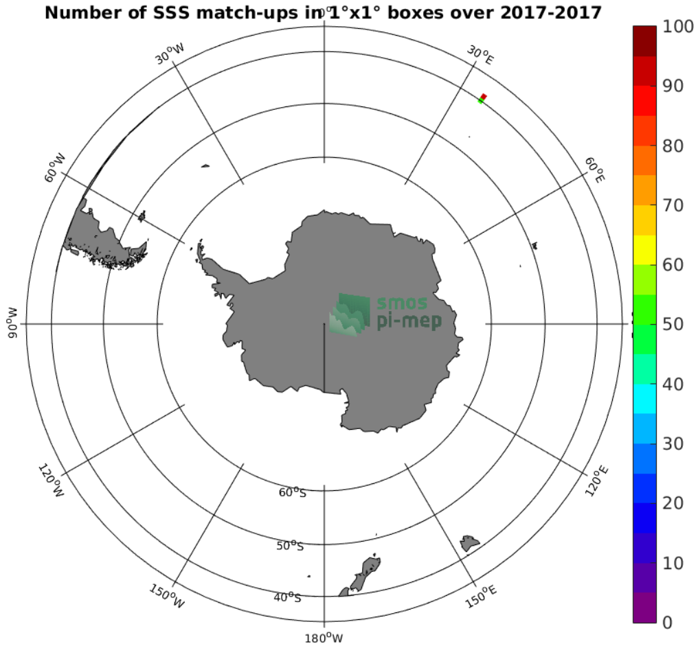
Figure 4: Number of SSS match-ups between TSG (GOSUD-Research-vessel) SSS and the SMAP SSS L2 v4 (RSS) SSS product for the Roaring Forties and Furious Fifties Pi-MEP region over 1°x1° boxes and for the full satellite product period.
