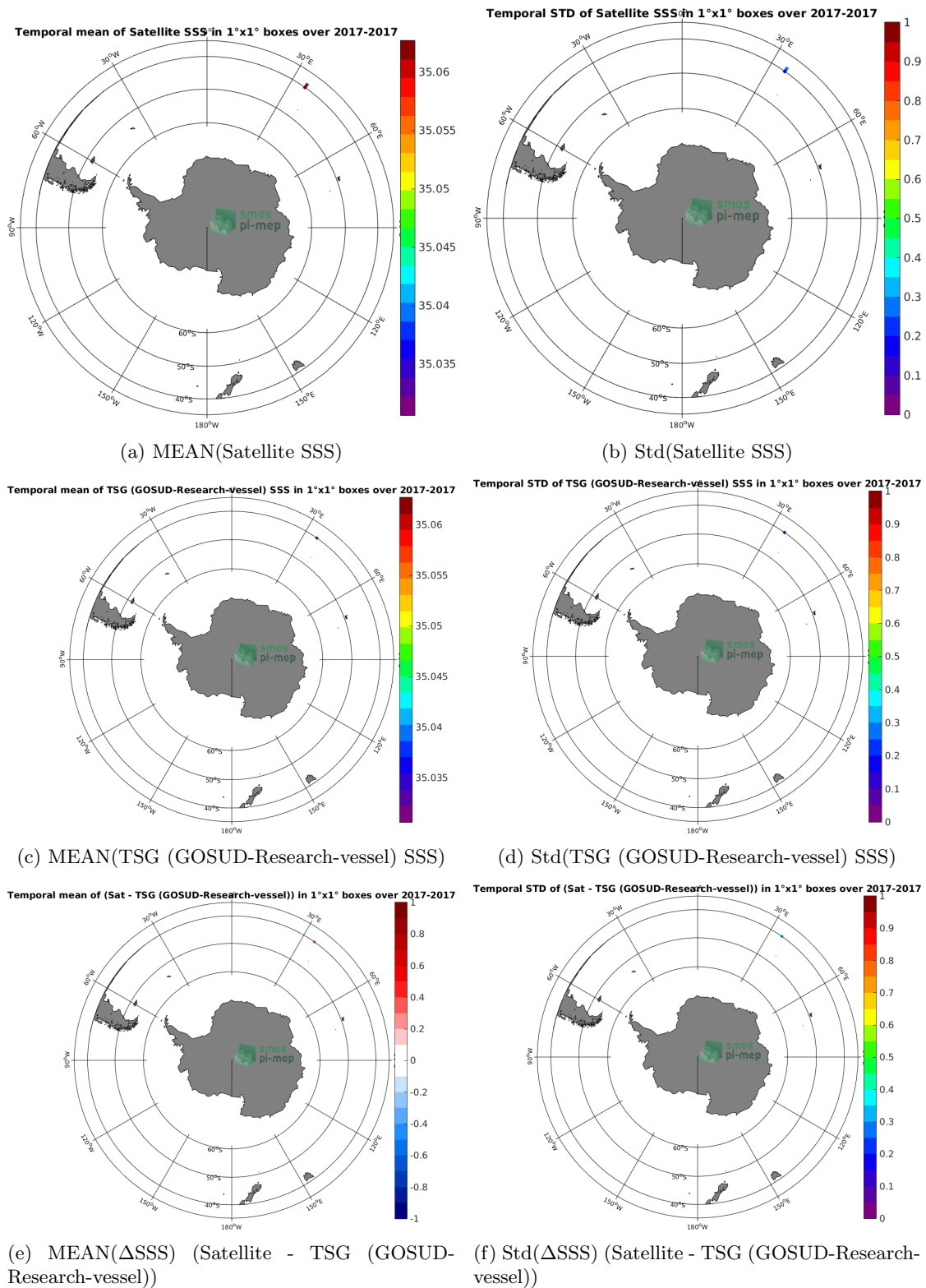
Figure 6: Temporal mean (left) and Std (right) of SSS from SMAP SSS L2 v4 (RSS) (top), TSG (GOSUD-Research-vessel) (middle), and of \Delta SSS (Satellite - TSG (GOSUD-Research-vessel)). Only match-up pairs are used to generate these maps.
