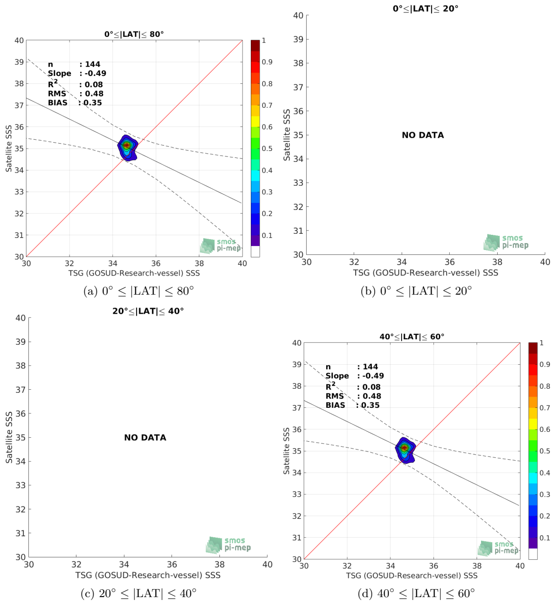
Figure 9: Contour maps of the concentration of SMAP SSS L2 v4 (RSS) SSS (y-axis) versus TSG (GOSUD-Research-vessel) SSS (x-axis) at match-up pairs for different latitude bands. For each plot, the red line shows x=y . The black thin and dashed lines indicate a linear fit through the data cloud and the \pm 95\% confidence levels, respectively. The number match-up pairs n , the slope and R^2 coefficient of the linear fit, the root mean square (RMS) and the mean bias between satellite and in situ data are indicated for each latitude band in each plots.
