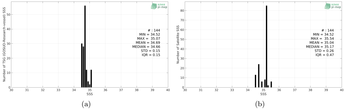
Figure 2: Histograms of SSS from TSG (GOSUD-Research-vessel) (a) and SMAP SSS L2 v4 (RSS) (b) considering all match-up pairs per bins of 0.1 over the Roaring Forties and Furious Fifties Pi-MEP region and for the full satellite product period.
