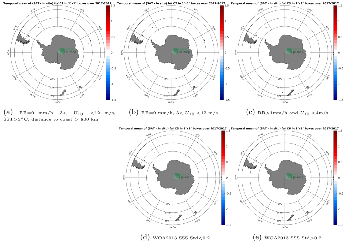
Figure 12: Temporal mean gridded over spatial boxes of size 1°x1° of \Delta SSS (SMAP SSS L2 v4 (RSS) - TSG (GOSUD-Research-vessel)) for 5 different subdatasets corresponding to:RR=0 mm/h, 3 < U_{10} < 12 m/s, SST > 5°C, distance to coast > 800 km (a), RR=0 mm/h, 3 < U_{10} < 12 m/s (b), RR > 1mm/h and U_{10} < 4 m/s (c), WOA2013 SSS Std < 0.2 (d), WOA2013 SSS Std > 0.2 (e).
