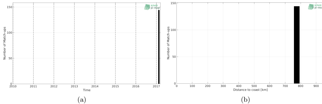
Figure 1: Number of match-ups between TSG (GOSUD-Research-vessel) and SMAP SSS L2 v4 (RSS) SSS as a function of time (a) and as function of the distance to coast (b) over the Roaring Forties and Furious Fifties Pi-MEP region and for the full satellite product period.
