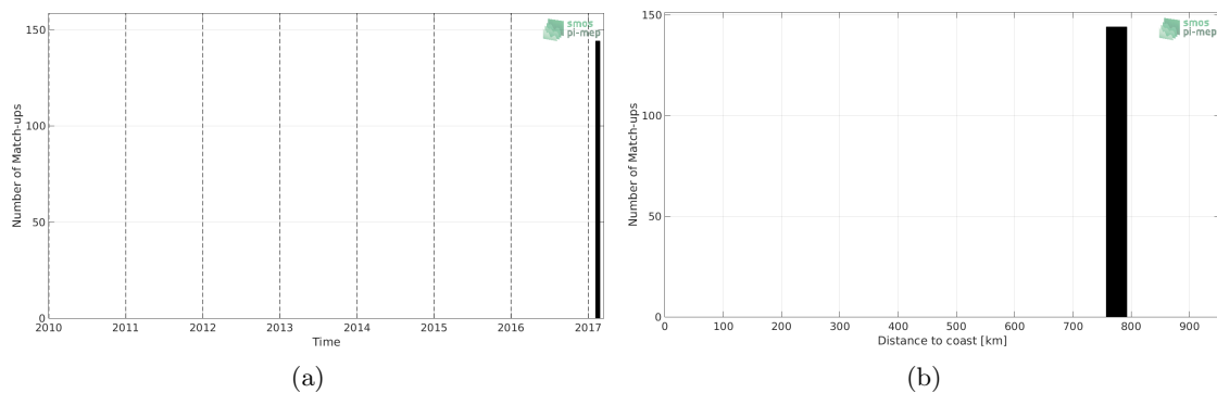
Figure 1: Number of match-ups between TSG-GOSUD-Research-vessel and SMAP-L2-RSS-V4 SSS as a function of time (a) and as function of the distance to coast (b) over the Roaring Forties and Furious Fifties Pi-MEP region and for the full satellite product period.
