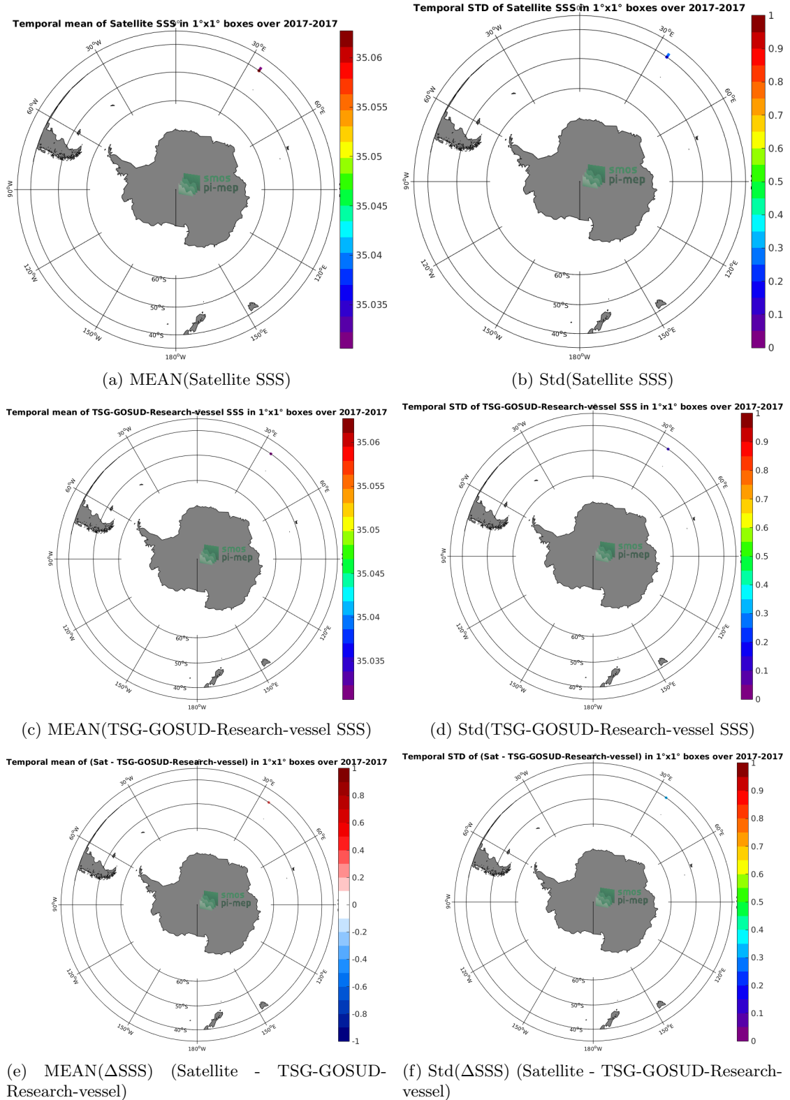
Figure 6: Temporal mean (left) and Std (right) of SSS from SMAP-L2-RSS-V4 (top), TSG-GOSUD-Research-vessel (middle), and of \Delta SSS (Satellite - TSG-GOSUD-Research-vessel). Only match-up pairs are used to generate these maps.
