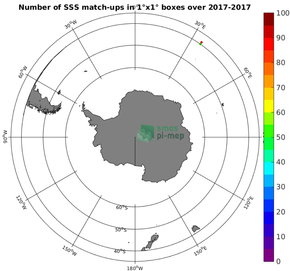
Figure 4: Number of SSS match-ups between TSG-GOSUD-Research-vessel SSS and the SMAP-L2-RSS-V4 SSS product for the Roaring Forties and Furious Fifties Pi-MEP region over 1°x1° boxes and for the full satellite product period.
