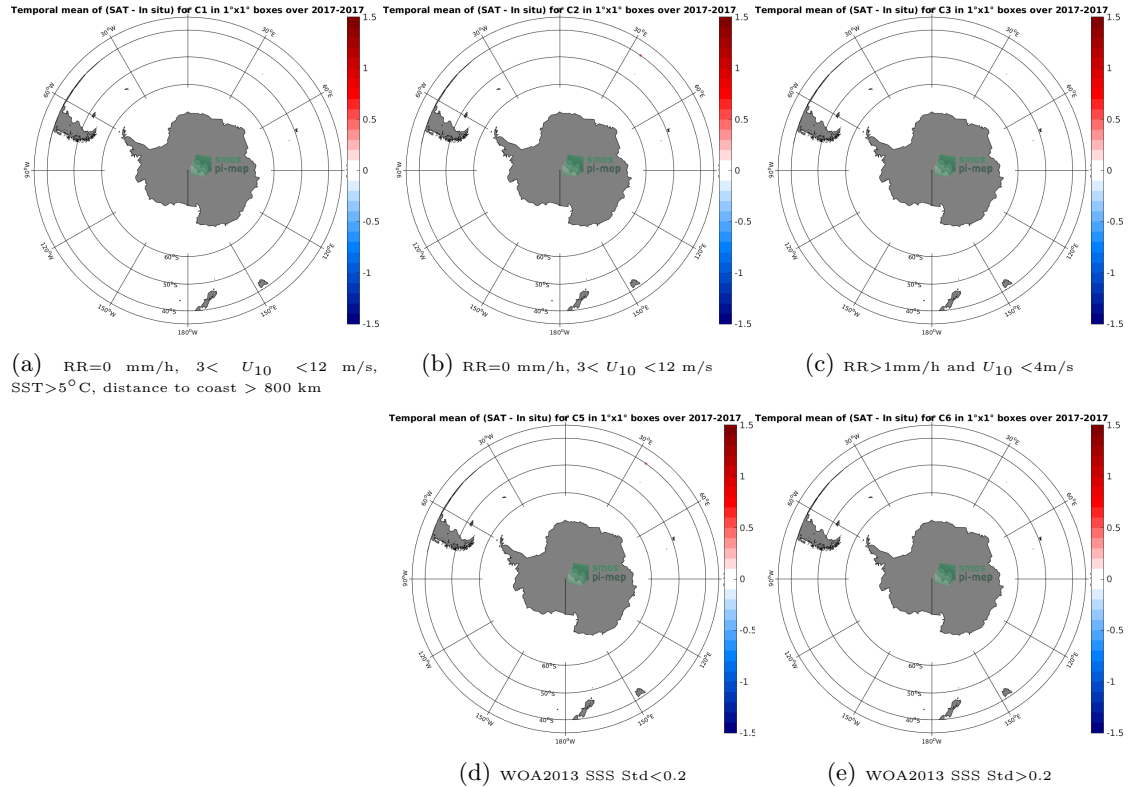
Figure 12: Temporal mean gridded over spatial boxes of size 1^\circ \times 1^\circ of \Delta SSS (SMAP-L2-RSS-V4 - TSG-GOSUD-Research-vessel) for 5 different subdatasets corresponding to: RR=0 mm/h, 3 < U_{10} < 12 m/s, SST > 5^\circ\text{C} , distance to coast > 800 km (a), RR=0 mm/h, 3 < U_{10} < 12 m/s (b), RR > 1 mm/h and U_{10} < 4 m/s (c), WOA2013 SSS Std < 0.2 (d), WOA2013 SSS Std > 0.2 (e).
