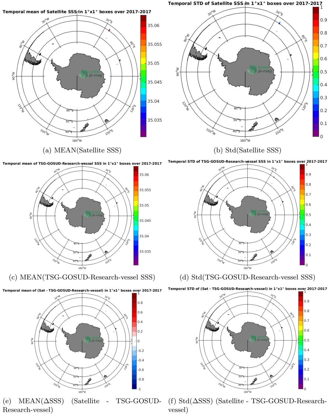
Figure 6: Temporal mean (left) and Std (right) of SSS from SMAP-L2-RSS-V4 (top), TSG-GOSUD-Research-vessel (middle), and of \Delta SSS (Satellite - TSG-GOSUD-Research-vessel). Only match-up pairs are used to generate these maps.
