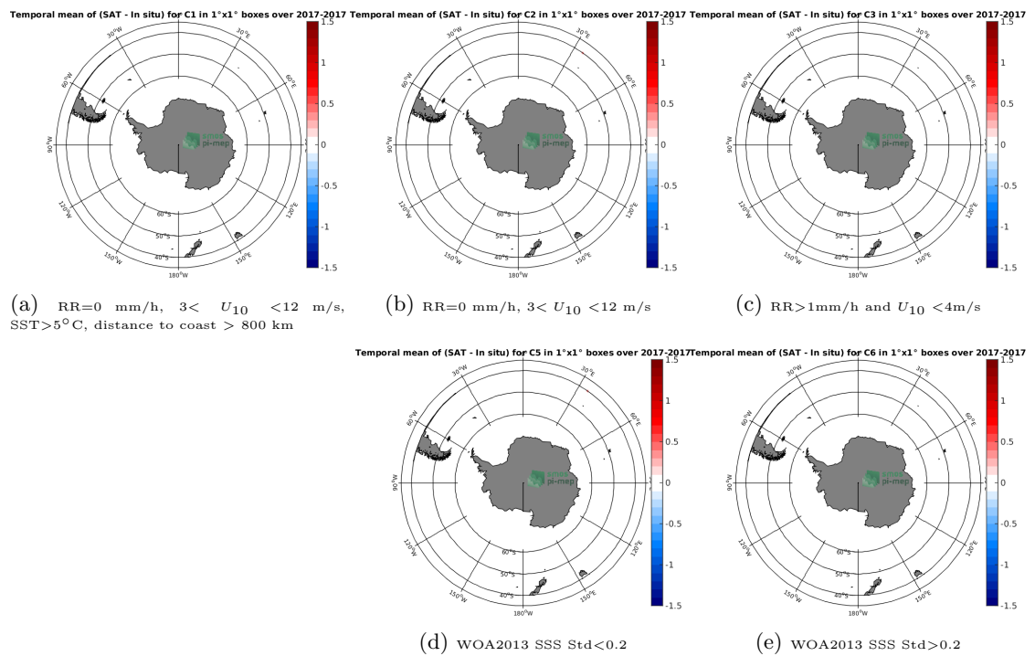
Figure 12: Temporal mean gridded over spatial boxes of size 1^\circ \times 1^\circ of \Delta SSS (SMAP-L2-RSS-V4 - TSG-GOSUD-Research-vessel) for 5 different subdatasets corresponding to:RR=0 mm/h, 3 < U_{10} < 12 m/s, SST>5°C, distance to coast > 800 km (a), RR=0 mm/h, 3 < U_{10} < 12 m/s (b), RR>1mm/h and U_{10} < 4 m/s (c), WOA2013 SSS Std<0.2 (d), WOA2013 SSS Std>0.2 (e).
