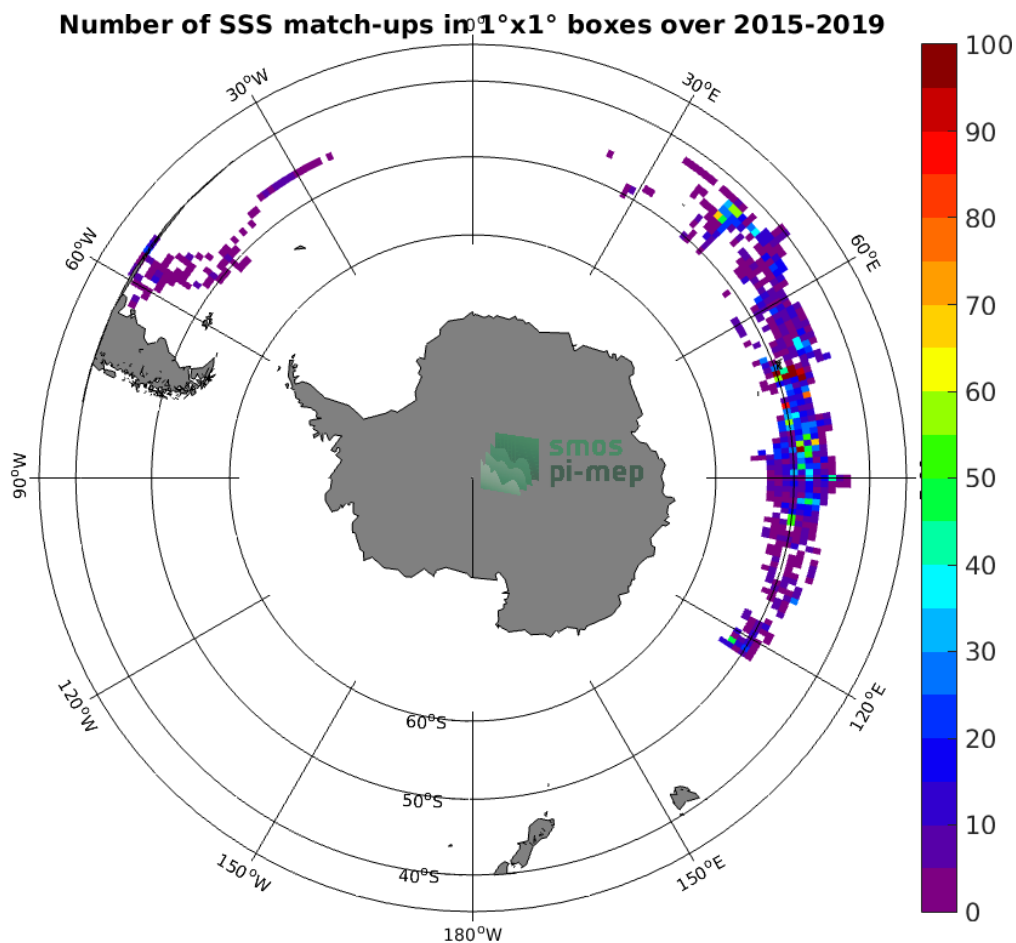
Figure 4: Number of SSS match-ups between Marine mammals SSS and the SMAP SSS L2 v4 (RSS) SSS product for the Roaring Forties and Furious Fifties Pi-MEP region over 1^\circ \times 1^\circ boxes and for the full satellite product period.
