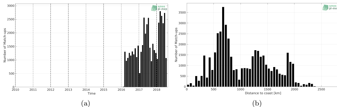
Figure 1: Number of match-ups between Surface drifters and SMAP SSS L2 v4 (RSS) SSS as a function of time (a) and as function of the distance to coast (b) over the Roaring Forties and Furious Fifties Pi-MEP region and for the full satellite product period.
