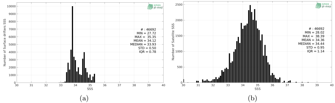
Figure 2: Histograms of SSS from Surface drifters (a) and SMAP SSS L2 v4 (RSS) (b) considering all match-up pairs per bins of 0.1 over the Roaring Forties and Furious Fifties Pi-MEP region and for the full satellite product period.
