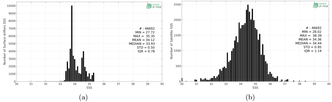
Figure 2: Histograms of SSS from Surface drifters (a) and SMAP SSS L2 v4 (RSS) (b) considering all match-up pairs per bins of 0.1 over the Roaring Forties and Furious Fifties Pi-MEP region and for the full satellite product period.
