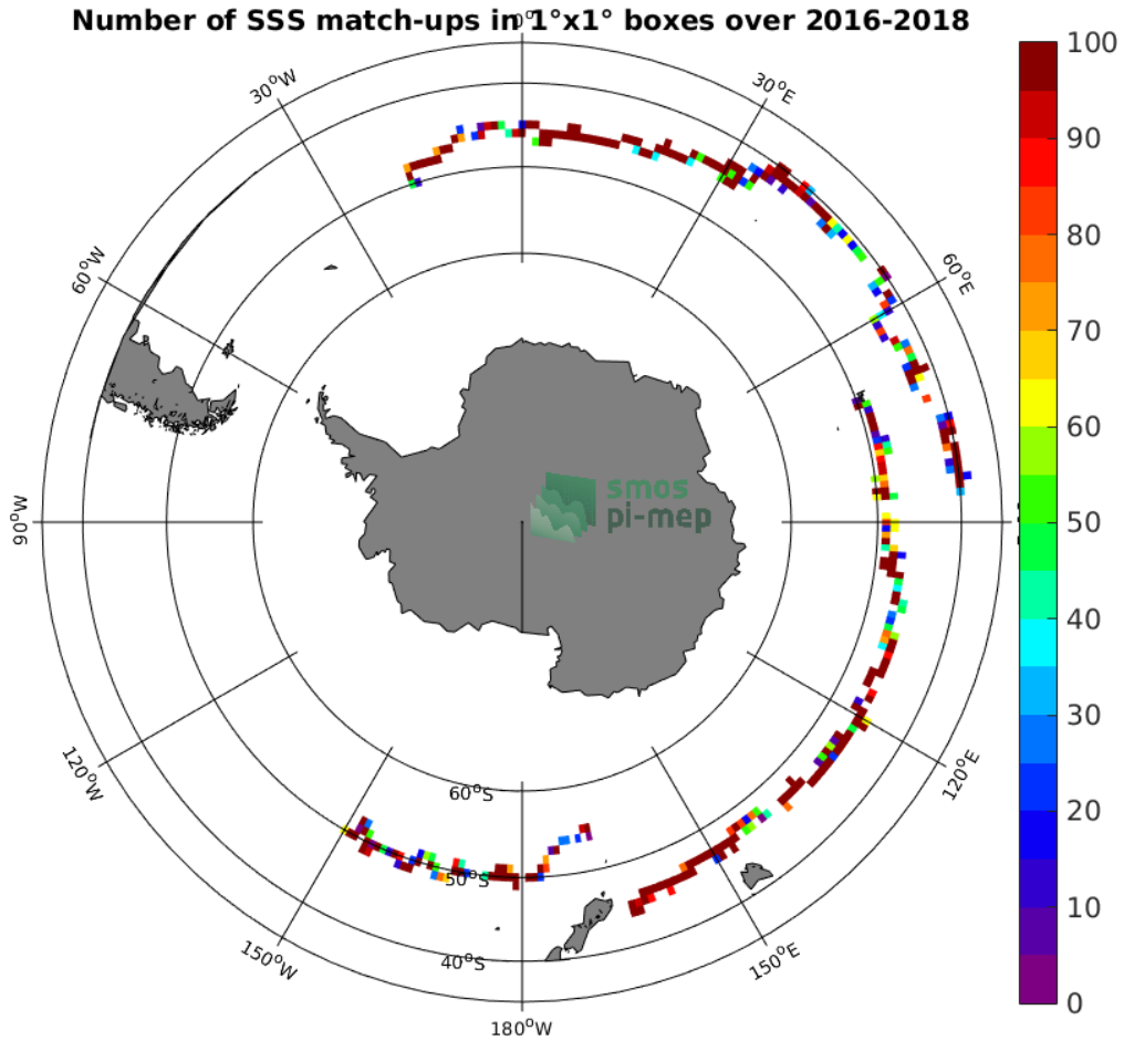
Figure 3: Number of SSS match-ups between Surface drifters SSS and the SMAP SSS L2 v4 (RSS) SSS product for the Roaring Forties and Furious Fifties Pi-MEP region over 1°x1° boxes and for the full satellite product period.
