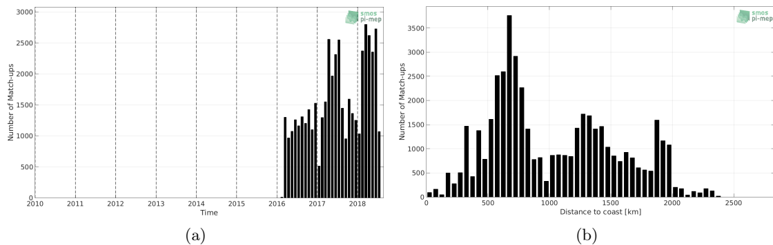
Figure 1: Number of match-ups between Surface drifters and SMAP-L2-RSS-V4 SSS as a function of time (a) and as function of the distance to coast (b) over the Roaring Forties and Furious Fifties Pi-MEP region and for the full satellite product period.
