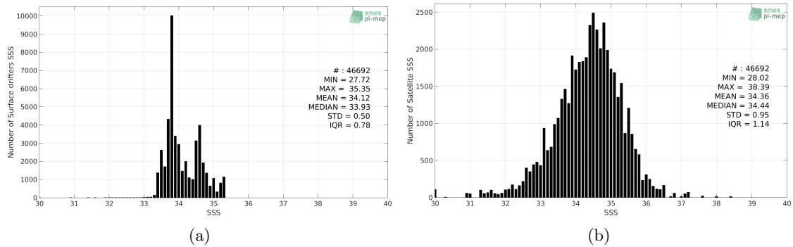
Figure 2: Histograms of SSS from Surface drifters (a) and SMAP-L2-RSS-V4 (b) considering all match-up pairs per bins of 0.1 over the Roaring Forties and Furious Fifties Pi-MEP region and for the full satellite product period.
