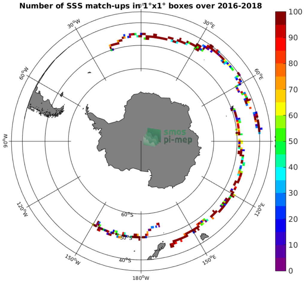
Figure 3: Number of SSS match-ups between Surface drifters SSS and the SMAP-L2-RSS-V4 SSS product for the Roaring Forties and Furious Fifties Pi-MEP region over 1°x1° boxes and for the full satellite product period.
