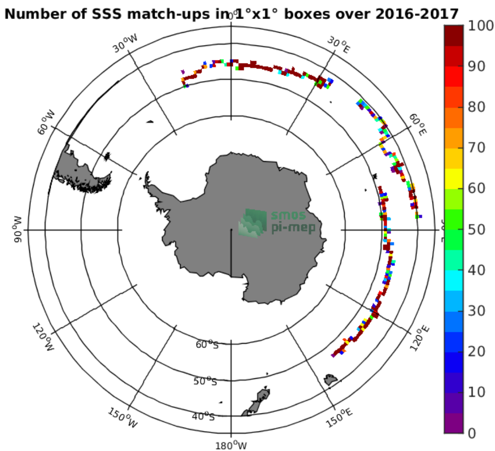
Figure 3: Number of SSS match-ups between Surface drifters SSS and the SMAP-L2-RSS-V4 SSS product for the Roaring Forties and Furious Fifties Pi-MEP region over 1^\circ \times 1^\circ boxes and for the full satellite product period.
