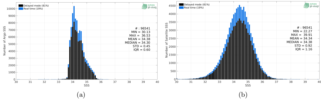
Figure 2: Histograms of SSS from Argo (a) and SMAP SSS L2 v4 (RSS) (b) considering all match-up pairs per bins of 0.1 over the Roaring Forties and Furious Fifties Pi-MEP region and for the full satellite product period.
