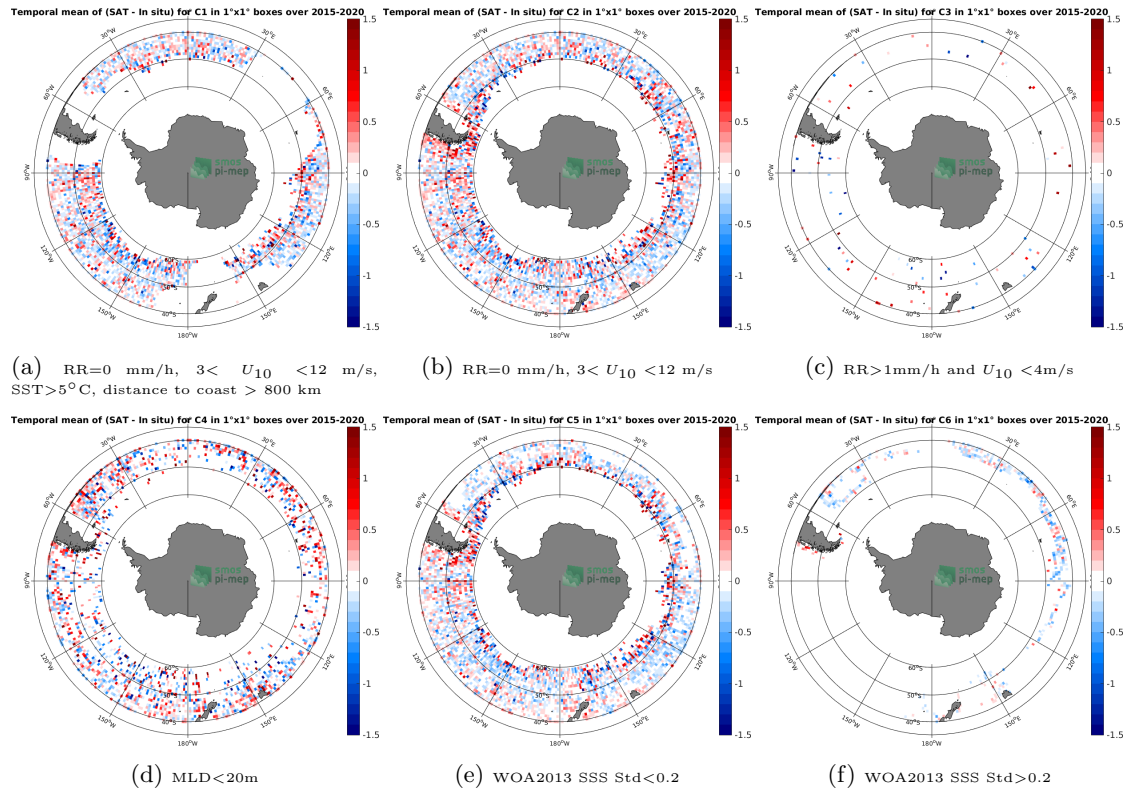
Figure 12: Temporal mean gridded over spatial boxes of size 1^{\circ}\times 1^{\circ} of \Delta\text{SSS} (SMAP-L2-RSS-V4 - Argo) for 6 different subdatasets corresponding to:RR=0 mm/h, 3 < U_{10} < 12 m/s, SST >5^{\circ}\text{C} , distance to coast > 800 km (a), RR=0 mm/h, 3 < U_{10} < 12 m/s (b), RR >1 mm/h and U_{10} < 4 m/s (c),MLD <20 m (d),WOA2013 SSS Std <0.2 (e),WOA2013 SSS Std >0.2 (f).
