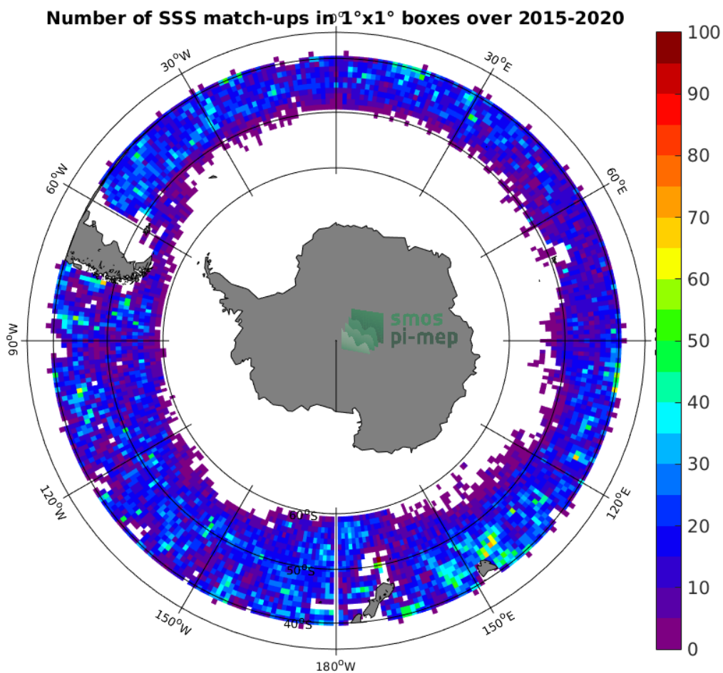
Figure 4: Number of SSS match-ups between Argo SSS and the SMAP-L2-RSS-V4 SSS product for the Roaring Forties and Furious Fifties Pi-MEP region over 1°x1° boxes and for the full satellite product period.
