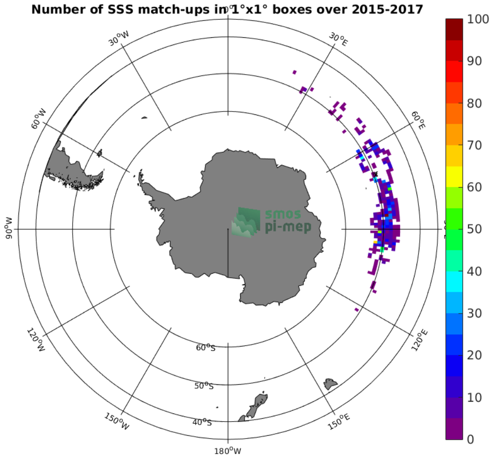
Figure 4: Number of SSS match-ups between Sea mammals SSS and the SMAP-L2-RSS-V3-70KM SSS product for the Roaring Forties and Furious Fifties Pi-MEP region over 1^\circ \times 1^\circ boxes and for the full satellite product period.
