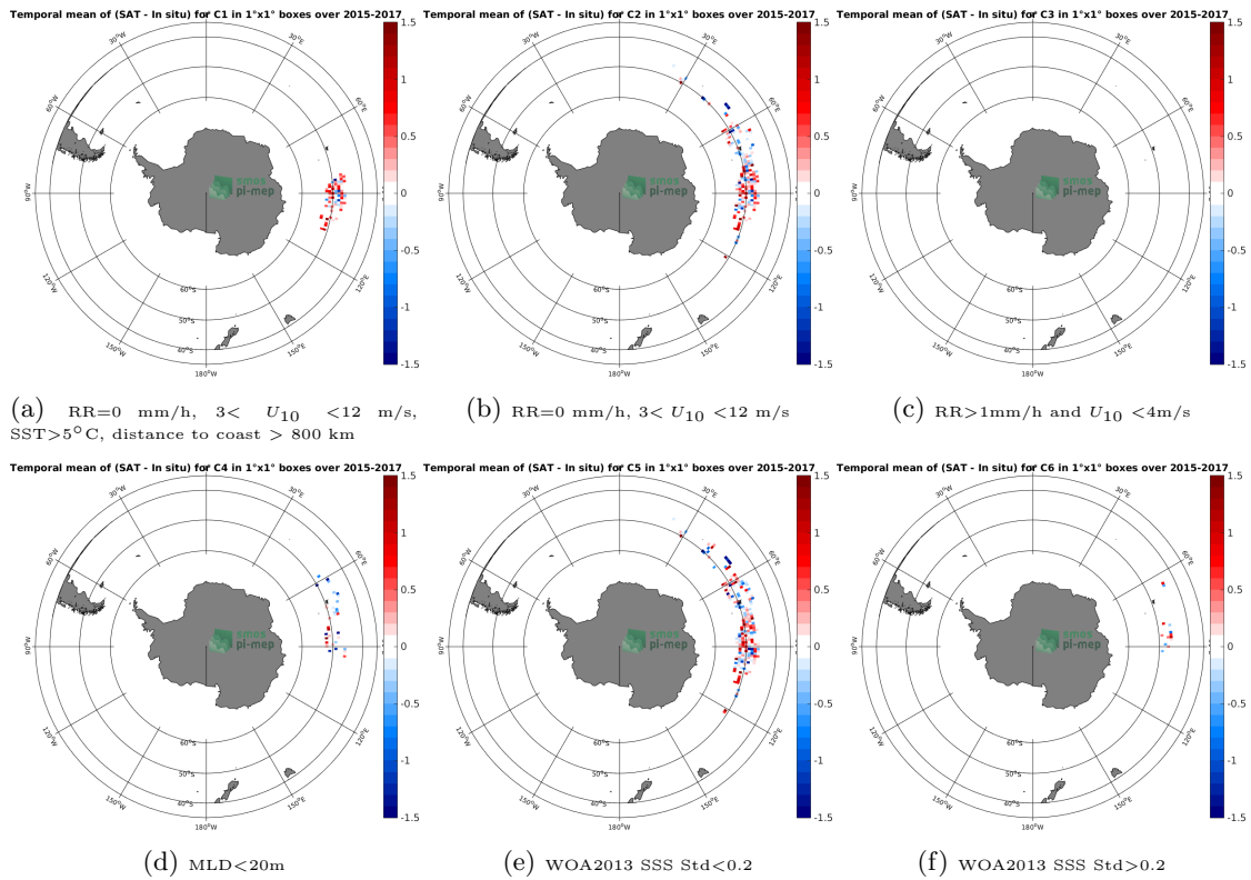
Figure 12: Temporal mean gridded over spatial boxes of size 1^\circ \times 1^\circ of \Delta SSS (SMAP-L2-RSS-V3-70KM - Sea mammals) for 6 different subdatasets corresponding to:RR=0 mm/h, 3 < U_{10} < 12 m/s, SST >5^\circ C, distance to coast > 800 km (a), RR=0 mm/h, 3 < U_{10} < 12 m/s (b), RR >1 mm/h and U_{10} < 4 m/s (c),MLD <20 m (d),WOA2013 SSS Std <0.2 (e),WOA2013 SSS Std >0.2 (f).
