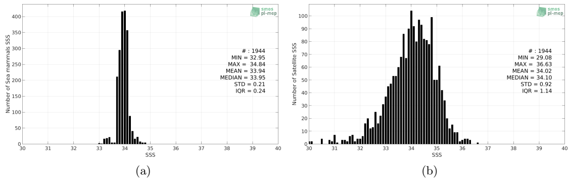
Figure 2: Histograms of SSS from Sea mammals (a) and SMAP-L2-RSS-V3-70KM (b) considering all match-up pairs per bins of 0.1 over the Roaring Forties and Furious Fifties Pi-MEP region and for the full satellite product period.
