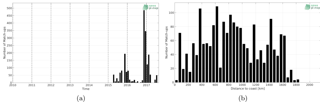
Figure 1: Number of match-ups between Sea mammals and SMAP-L2-RSS-V3-70KM SSS as a function of time (a) and as function of the distance to coast (b) over the Roaring Forties and Furious Fifties Pi-MEP region and for the full satellite product period.
