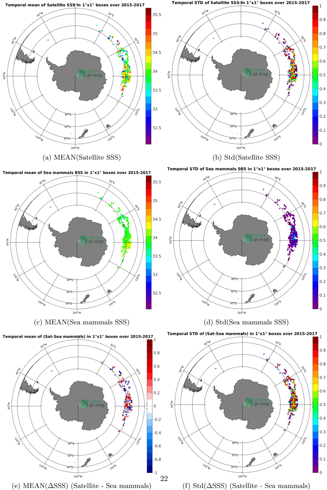
Figure 6: Temporal mean (left) and Std (right) of SSS from SMAP-L2-RSS-V3-70KM (top), Sea mammals (middle), and of \Delta SSS (Satellite - Sea mammals). Only match-up pairs are used to generate these maps.
