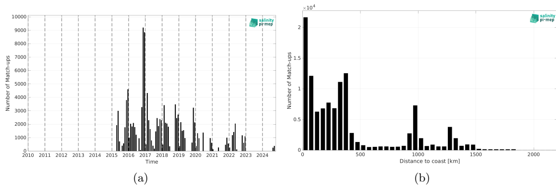
Figure 2: Number of match-ups between TSG (SAMOS) and SMAP SSS L2 v5.0 (JPL) SSS as a function of time (a) and as function of the distance to coast (b) over the Roaring Forties and Furious Fifties Pi-MEP region and for the full satellite product period.
