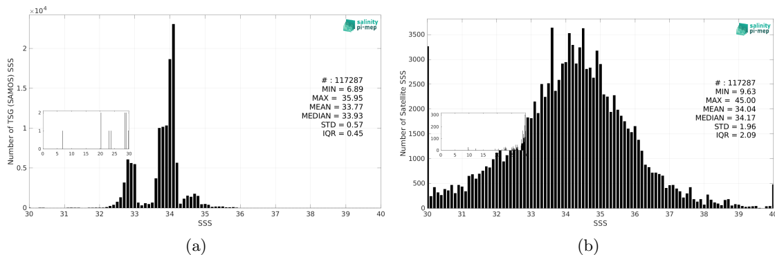
Figure 3: Histograms of SSS from TSG (SAMOS) (a) and SMAP SSS L2 v5.0 (JPL) (b) considering all match-up pairs per bins of 0.1 over the Roaring Forties and Furious Fifties Pi-MEP region and for the full satellite product period.
