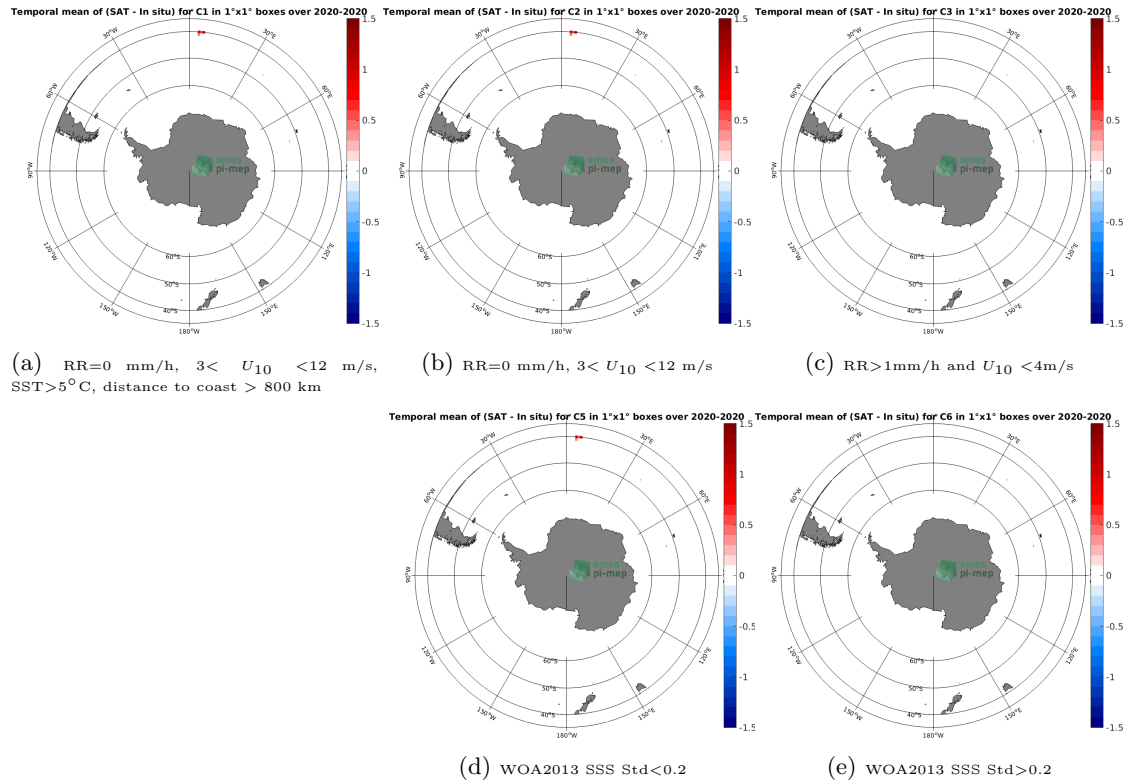
Figure 12: Temporal mean gridded over spatial boxes of size 1^{\circ}\times 1^{\circ} of \Delta\text{SSS} (SMAP SSS L2 v5.0 (JPL) - TSG (SAMOS)) for 5 different subdatasets corresponding to:RR=0 mm/h, 3 < U_{10} < 12 m/s, SST >5^{\circ}\text{C} , distance to coast > 800 km (a), RR=0 mm/h, 3 < U_{10} < 12 m/s (b), RR >1 mm/h and U_{10} < 4 m/s (c), WOA2013 SSS Std <0.2 (d), WOA2013 SSS Std >0.2 (e).
