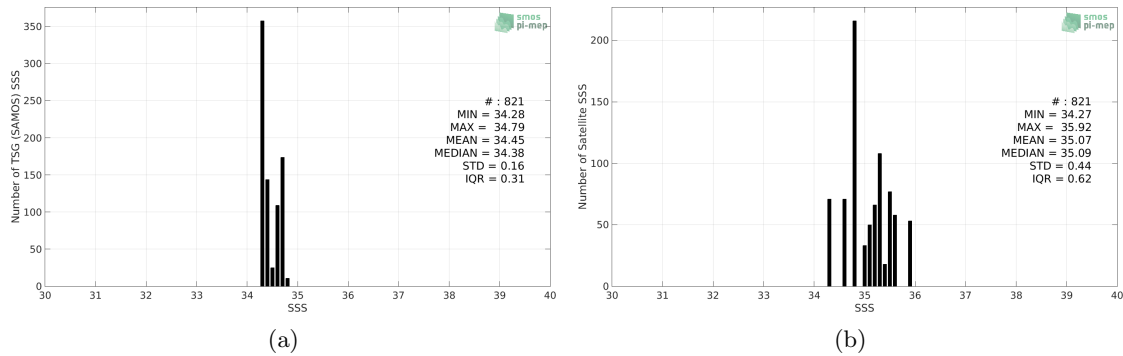
Figure 2: Histograms of SSS from TSG (SAMOS) (a) and SMAP SSS L2 v5.0 (JPL) (b) considering all match-up pairs per bins of 0.1 over the Roaring Forties and Furious Fifties Pi-MEP region and for the full satellite product period.
