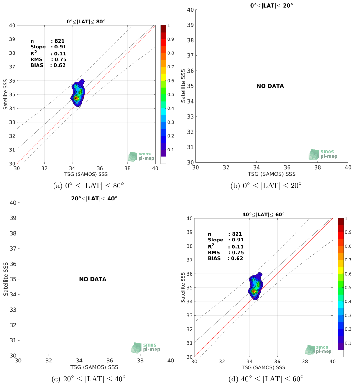
Figure 9: Contour maps of the concentration of SMAP SSS L2 v5.0 (JPL) SSS (y-axis) versus TSG (SAMOS) SSS (x-axis) at match-up pairs for different latitude bands. For each plot, the red line shows x=y . The black thin and dashed lines indicate a linear fit through the data cloud and the \pm 95\% confidence levels, respectively. The number match-up pairs n , the slope and R^2 coefficient of the linear fit, the root mean square (RMS) and the mean bias between satellite and in situ data are indicated for each latitude band in each plots.
