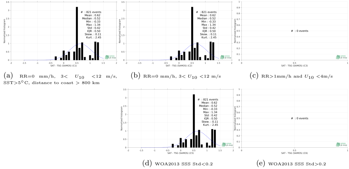
Figure 13: Normalized histogram of \Delta\text{SSS} (SMAP SSS L2 v5.0 (JPL) - TSG (SAMOS)) for 5 different subdatasets corresponding to: RR=0 mm/h, 3 < U_{10} < 12 m/s, SST>5°C, distance to coast > 800 km (a), RR=0 mm/h, 3 < U_{10} < 12 m/s (b), RR>1mm/h and U_{10} < 4 m/s (c), WOA2013 SSS Std<0.2 (d), WOA2013 SSS Std>0.2 (e).
