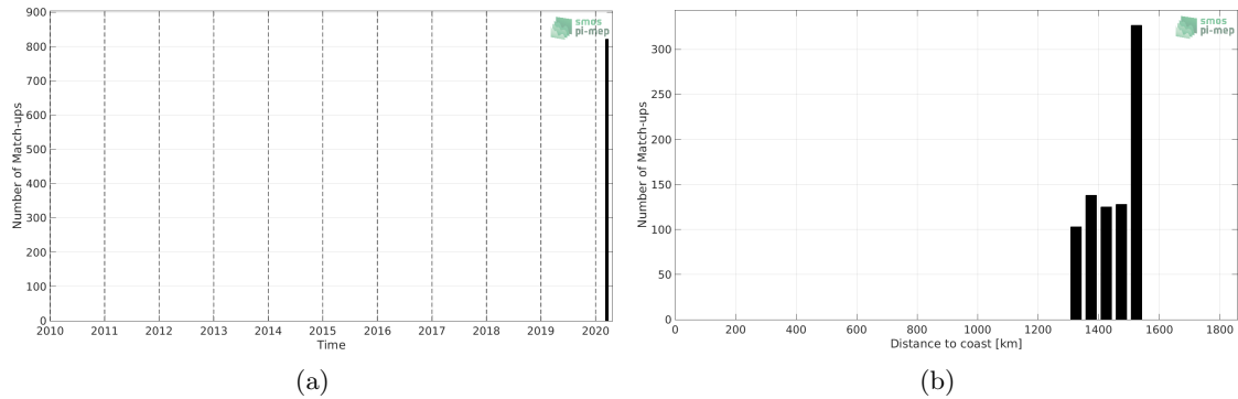
Figure 1: Number of match-ups between TSG (SAMOS) and SMAP SSS L2 v5.0 (JPL) SSS as a function of time (a) and as function of the distance to coast (b) over the Roaring Forties and Furious Fifties Pi-MEP region and for the full satellite product period.
