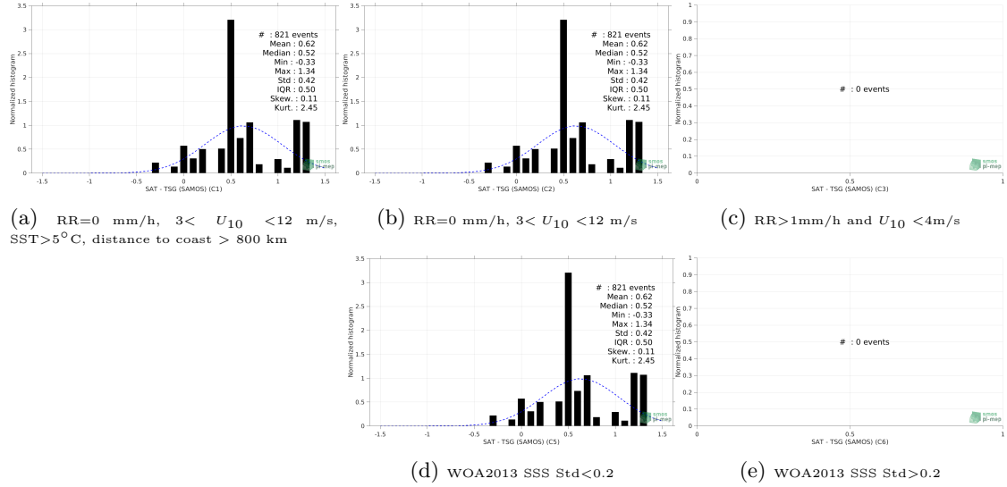
Figure 13: Normalized histogram of \Delta\text{SSS} (SMAP SSS L2 v5.0 (JPL) - TSG (SAMOS)) for 5 different subdatasets corresponding to: RR=0 mm/h, 3 < U_{10} < 12 m/s, SST > 5^\circ\text{C} , distance to coast > 800 km (a), RR=0 mm/h, 3 < U_{10} < 12 m/s (b), RR > 1\text{mm/h} and U_{10} < 4\text{m/s} (c), WOA2013 SSS Std < 0.2 (d), WOA2013 SSS Std > 0.2 (e).
