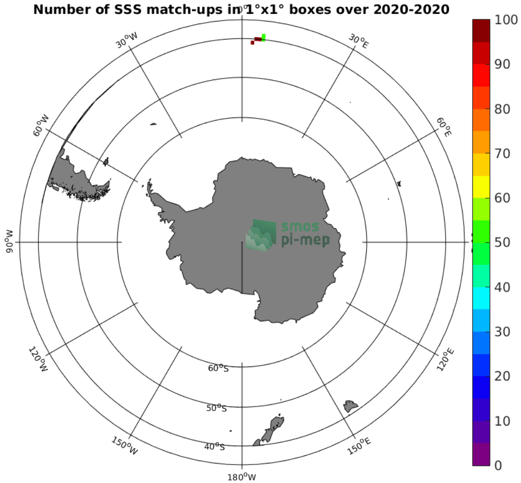
Figure 4: Number of SSS match-ups between TSG (SAMOS) SSS and the SMAP SSS L2 v5.0 (JPL) SSS product for the Roaring Forties and Furious Fifties Pi-MEP region over 1°x1° boxes and for the full satellite product period.
