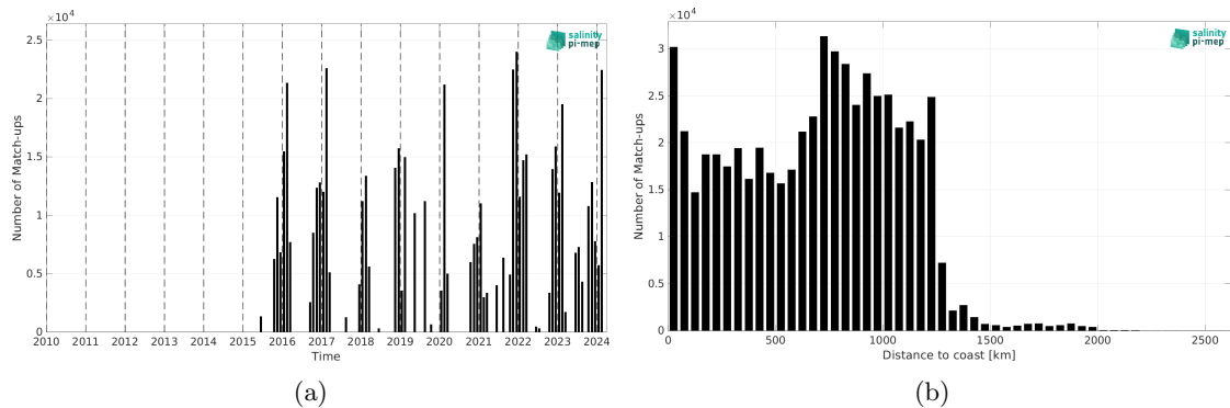
Figure 2: Number of match-ups between TSG (LEGOS-DM) and SMAP SSS L2 v5.0 (JPL) SSS as a function of time (a) and as function of the distance to coast (b) over the Roaring Forties and Furious Fifties Pi-MEP region and for the full satellite product period.
