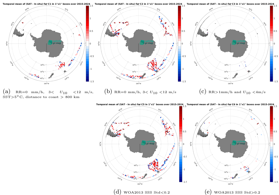
Figure 14: Temporal mean gridded over spatial boxes of size 1^\circ \times 1^\circ of \Delta SSS (SMAP SSS L2 v5.0 (JPL) - TSG (LEGOS-DM)) for 5 different subdatasets corresponding to:RR=0 mm/h, 3 < U_{10} < 12 m/s, SST>5°C, distance to coast > 800 km (a), RR=0 mm/h, 3 < U_{10} < 12 m/s (b), RR>1mm/h and U_{10} < 4 m/s (c), WOA2013 SSS Std<0.2 (d), WOA2013 SSS Std>0.2 (e).
