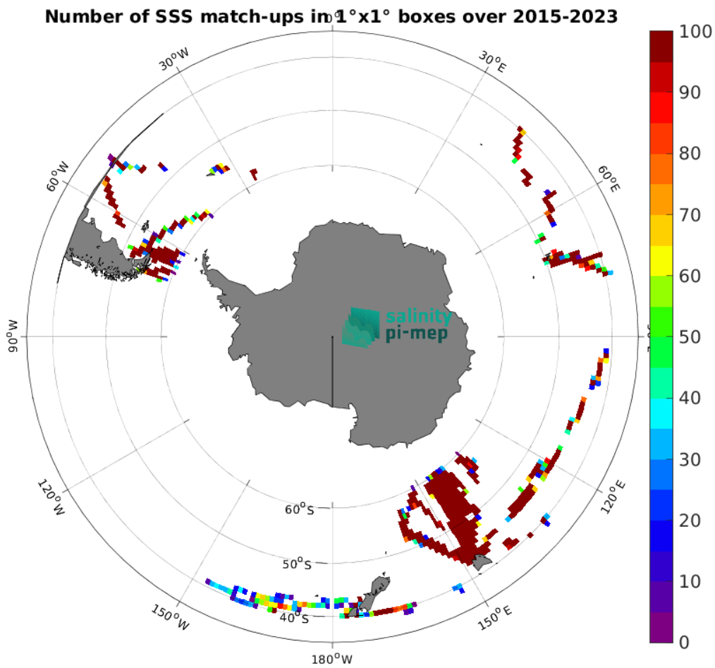
Figure 5: Number of SSS match-ups between TSG (LEGOS-DM) SSS and the SMAP SSS L2 v5.0 (JPL) SSS product for the Roaring Forties and Furious Fifties Pi-MEP region over 1^\circ \times 1^\circ boxes and for the full satellite product period.
