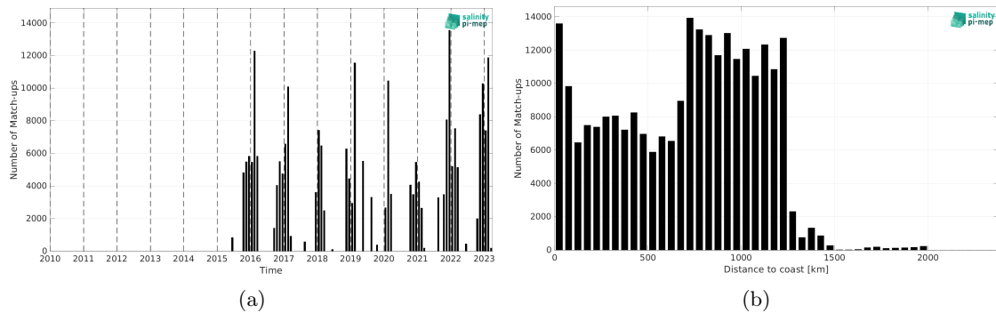
Figure 2: Number of match-ups between TSG (LEGOS-DM) and SMAP SSS L2 v5.0 (JPL) SSS as a function of time (a) and as function of the distance to coast (b) over the Roaring Forties and Furious Fifties Pi-MEP region and for the full satellite product period.
