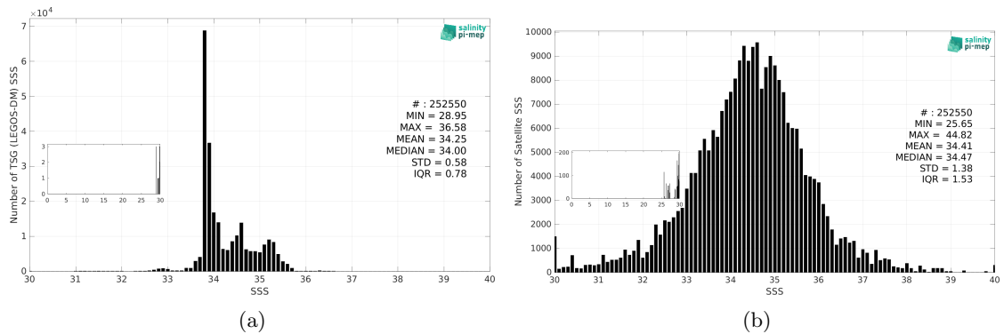
Figure 3: Histograms of SSS from TSG (LEGOS-DM) (a) and SMAP SSS L2 v5.0 (JPL) (b) considering all match-up pairs per bins of 0.1 over the Roaring Forties and Furious Fifties Pi-MEP region and for the full satellite product period.
