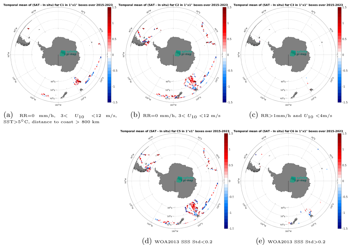
Figure 14: Temporal mean gridded over spatial boxes of size 1^\circ \times 1^\circ of \Delta\text{SSS} (SMAP SSS L2 v5.0 (JPL) - TSG (LEGOS-DM)) for 5 different subdatasets corresponding to:RR=0 mm/h, 3 < U_{10} < 12 m/s, SST>5°C, distance to coast > 800 km (a), RR=0 mm/h, 3 < U_{10} < 12 m/s (b), RR>1mm/h and U_{10} < 4 m/s (c), WOA2013 SSS Std<0.2 (d), WOA2013 SSS Std>0.2 (e).
