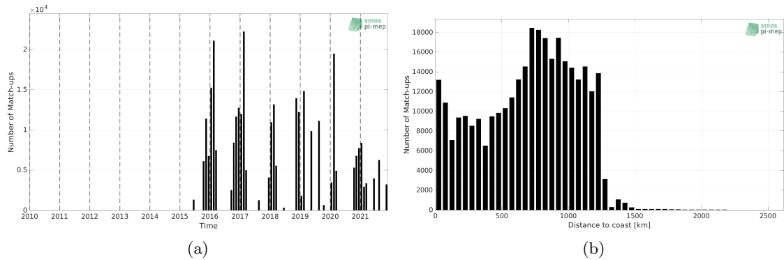
Figure 1: Number of match-ups between TSG (LEGOS-DM) and SMAP SSS L2 v5.0 (JPL) SSS as a function of time (a) and as function of the distance to coast (b) over the Roaring Forties and Furious Fifties Pi-MEP region and for the full satellite product period.
