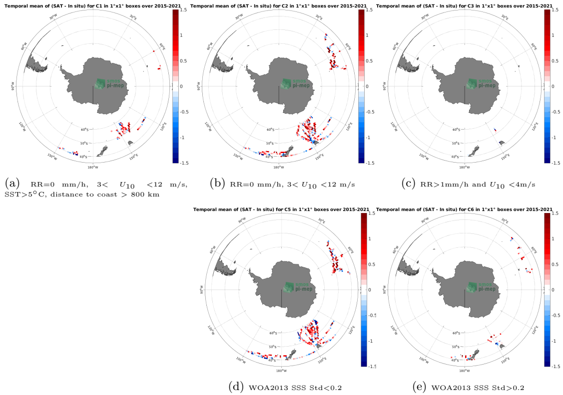
Figure 12: Temporal mean gridded over spatial boxes of size 1^{\circ}\times 1^{\circ} of \Delta\text{SSS} (SMAP SSS L2 v5.0 (JPL) - TSG (LEGOS-DM)) for 5 different subdatasets corresponding to: \text{RR}=0 mm/h, 3 < U_{10} < 12 m/s, \text{SST}>5^{\circ}\text{C} , distance to coast > 800 km (a), \text{RR}=0 mm/h, 3 < U_{10} < 12 m/s (b), \text{RR}>1\text{mm/h} and U_{10} < 4\text{m/s} (c), WOA2013 SSS Std < 0.2 (d), WOA2013 SSS Std > 0.2 (e).
