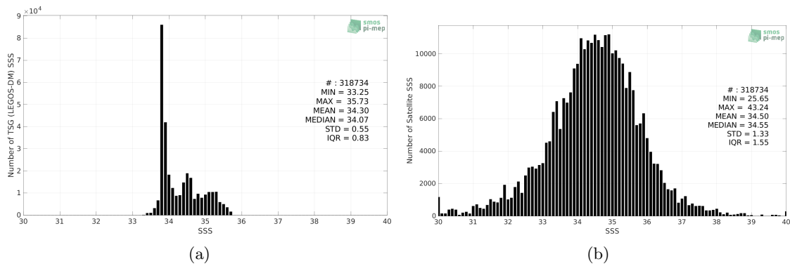
Figure 2: Histograms of SSS from TSG (LEGOS-DM) (a) and SMAP SSS L2 v5.0 (JPL) (b) considering all match-up pairs per bins of 0.1 over the Roaring Forties and Furious Fifties Pi-MEP region and for the full satellite product period.
