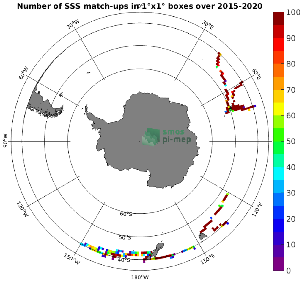
Figure 4: Number of SSS match-ups between TSG (LEGOS-DM) SSS and the SMAP SSS L2 v5.0 (JPL) SSS product for the Roaring Forties and Furious Fifties Pi-MEP region over 1^\circ \times 1^\circ boxes and for the full satellite product period.
