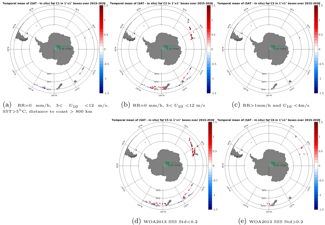
Figure 12: Temporal mean gridded over spatial boxes of size 1^{\circ}\times 1^{\circ} of \Delta\text{SSS} (SMAP SSS L2 v5.0 (JPL) - TSG (LEGOS-DM)) for 5 different subdatasets corresponding to:RR=0 mm/h, 3 < U_{10} < 12 m/s, SST >5^{\circ}\text{C} , distance to coast > 800 km (a), RR=0 mm/h, 3 < U_{10} < 12 m/s (b), RR >1 mm/h and U_{10} < 4 m/s (c), WOA2013 SSS Std <0.2 (d), WOA2013 SSS Std >0.2 (e).
