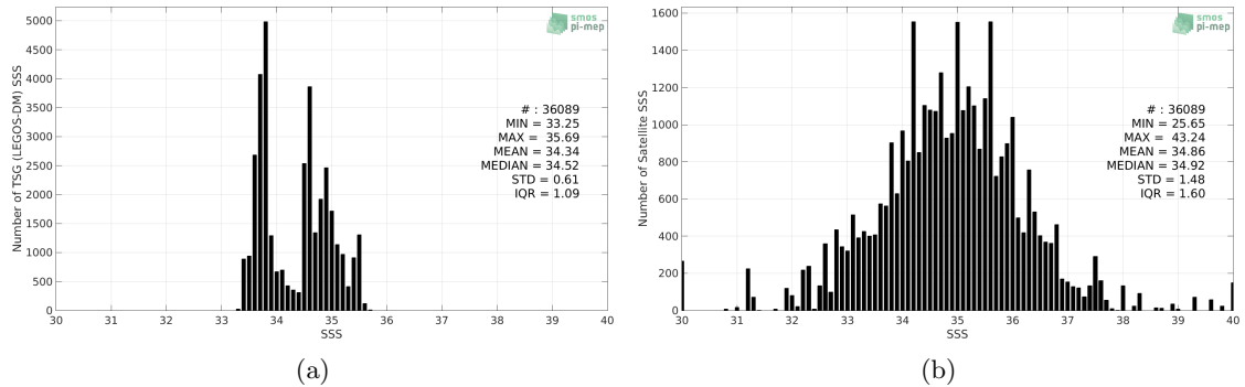
Figure 2: Histograms of SSS from TSG (LEGOS-DM) (a) and SMAP SSS L2 v5.0 (JPL) (b) considering all match-up pairs per bins of 0.1 over the Roaring Forties and Furious Fifties Pi-MEP region and for the full satellite product period.
