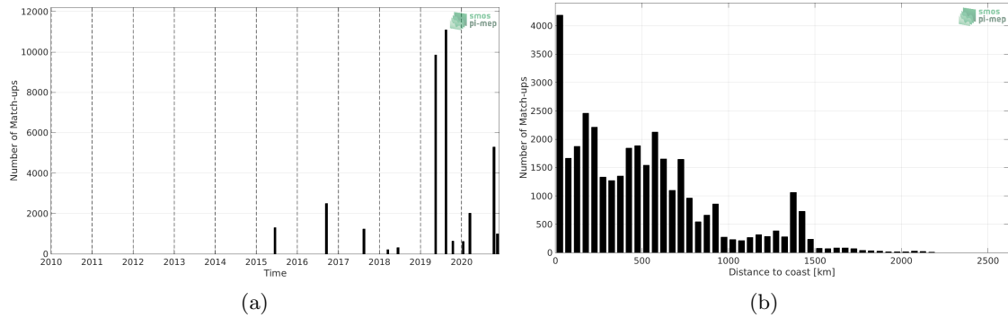
Figure 1: Number of match-ups between TSG (LEGOS-DM) and SMAP SSS L2 v5.0 (JPL) SSS as a function of time (a) and as function of the distance to coast (b) over the Roaring Forties and Furious Fifties Pi-MEP region and for the full satellite product period.
