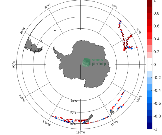
(e) MEAN( \Delta SSS) (Satellite - TSG (LEGOS-DM))
