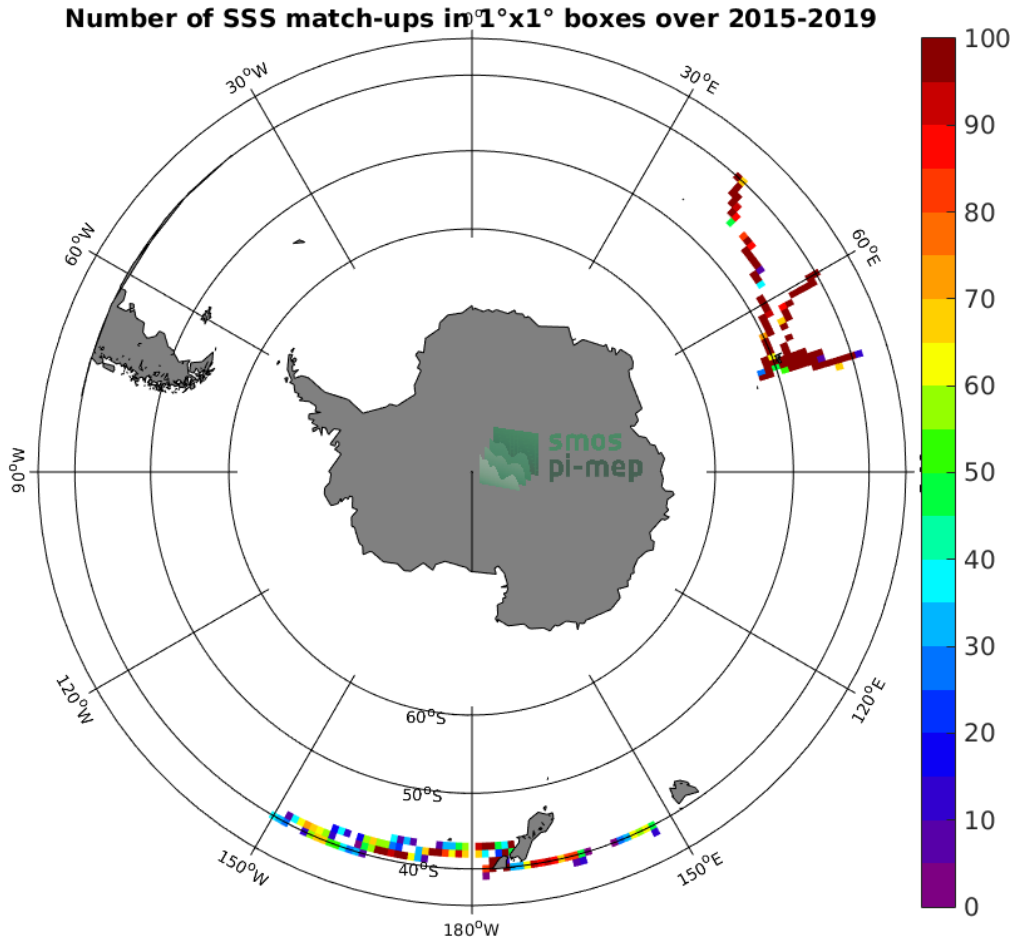
Figure 4: Number of SSS match-ups between TSG (LEGOS-DM) SSS and the SMAP SSS L2 v5.0 (JPL) SSS product for the Roaring Forties and Furious Fifties Pi-MEP region over 1°x1° boxes and for the full satellite product period.
