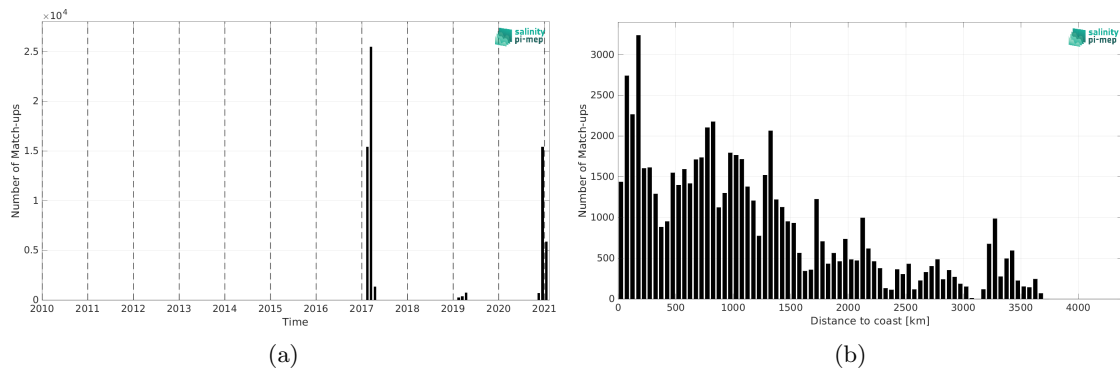
Figure 2: Number of match-ups between TSG (GOSUD-Sailing-ship) and SMAP SSS L2 v5.0 (JPL) SSS as a function of time (a) and as function of the distance to coast (b) over the Roaring Forties and Furious Fifties Pi-MEP region and for the full satellite product period.
