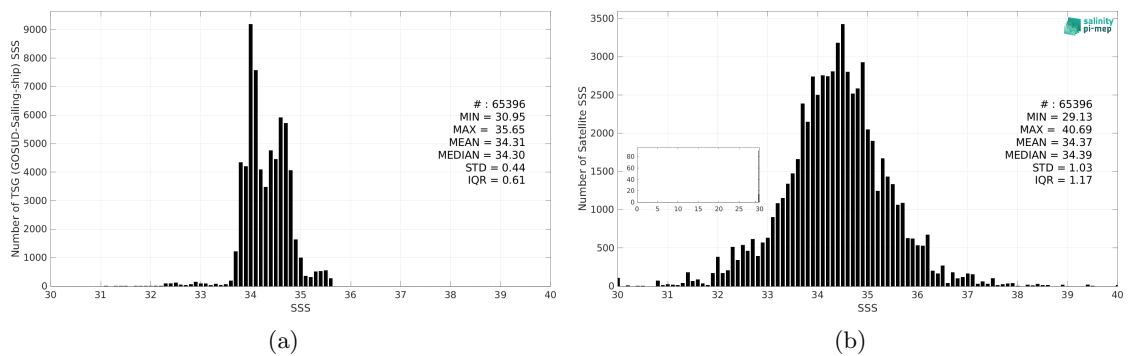
Figure 3: Histograms of SSS from TSG (GOSUD-Sailing-ship) (a) and SMAP SSS L2 v5.0 (JPL) (b) considering all match-up pairs per bins of 0.1 over the Roaring Forties and Furious Fifties Pi-MEP region and for the full satellite product period.
