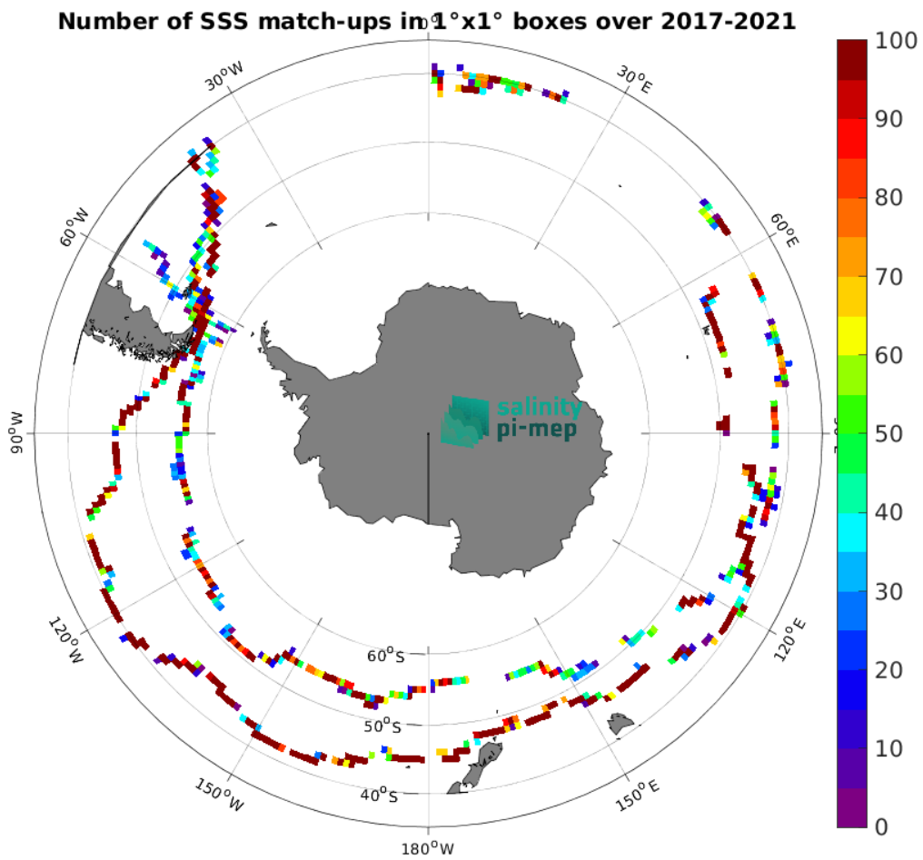
Figure 5: Number of SSS match-ups between TSG (GOSUD-Sailing-ship) SSS and the SMAP SSS L2 v5.0 (JPL) SSS product for the Roaring Forties and Furious Fifties Pi-MEP region over 1^\circ \times 1^\circ boxes and for the full satellite product period.
