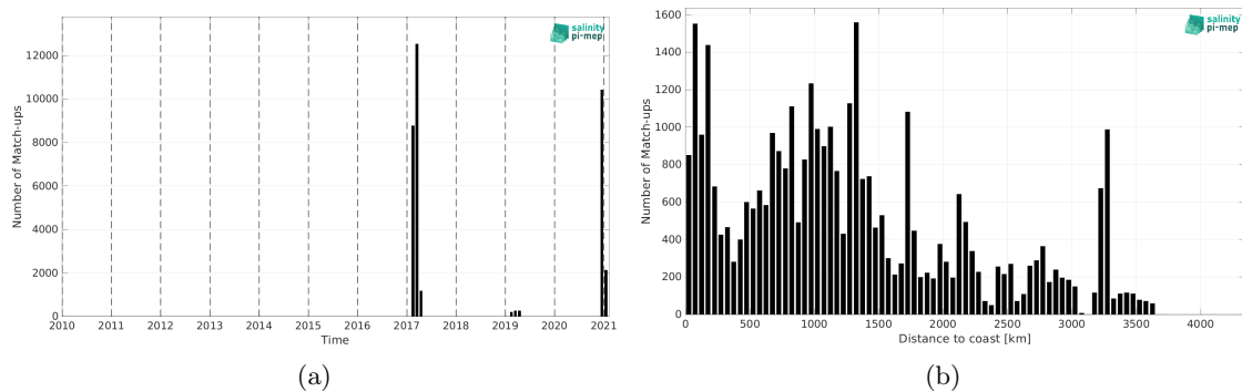
Figure 2: Number of match-ups between TSG (GOSUD-Sailing-ship) and SMAP SSS L2 v5.0 (JPL) SSS as a function of time (a) and as function of the distance to coast (b) over the Roaring Forties and Furious Fifties Pi-MEP region and for the full satellite product period.
