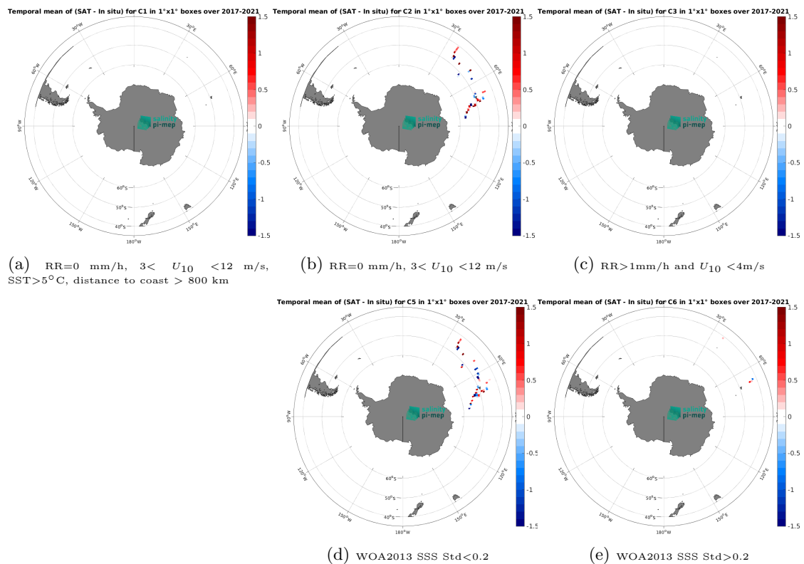
Figure 14: Temporal mean gridded over spatial boxes of size 1^\circ \times 1^\circ of \Delta SSS (SMAP SSS L2 v5.0 (JPL) - TSG (GOSUD-Research-vessel)) for 5 different subdatasets corresponding to:RR=0 mm/h, 3 < U_{10} < 12 m/s, SST>5°C, distance to coast > 800 km (a), RR=0 mm/h, 3 < U_{10} < 12 m/s (b), RR>1mm/h and U_{10} < 4 m/s (c), WOA2013 SSS Std<0.2 (d), WOA2013 SSS Std>0.2 (e).
