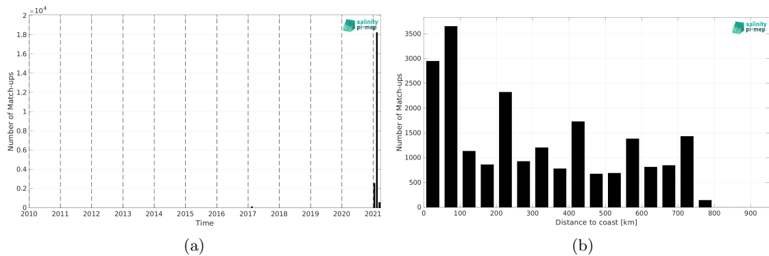
Figure 2: Number of match-ups between TSG (GOSUD-Research-vessel) and SMAP SSS L2 v5.0 (JPL) SSS as a function of time (a) and as function of the distance to coast (b) over the Roaring Forties and Furious Fifties Pi-MEP region and for the full satellite product period.
