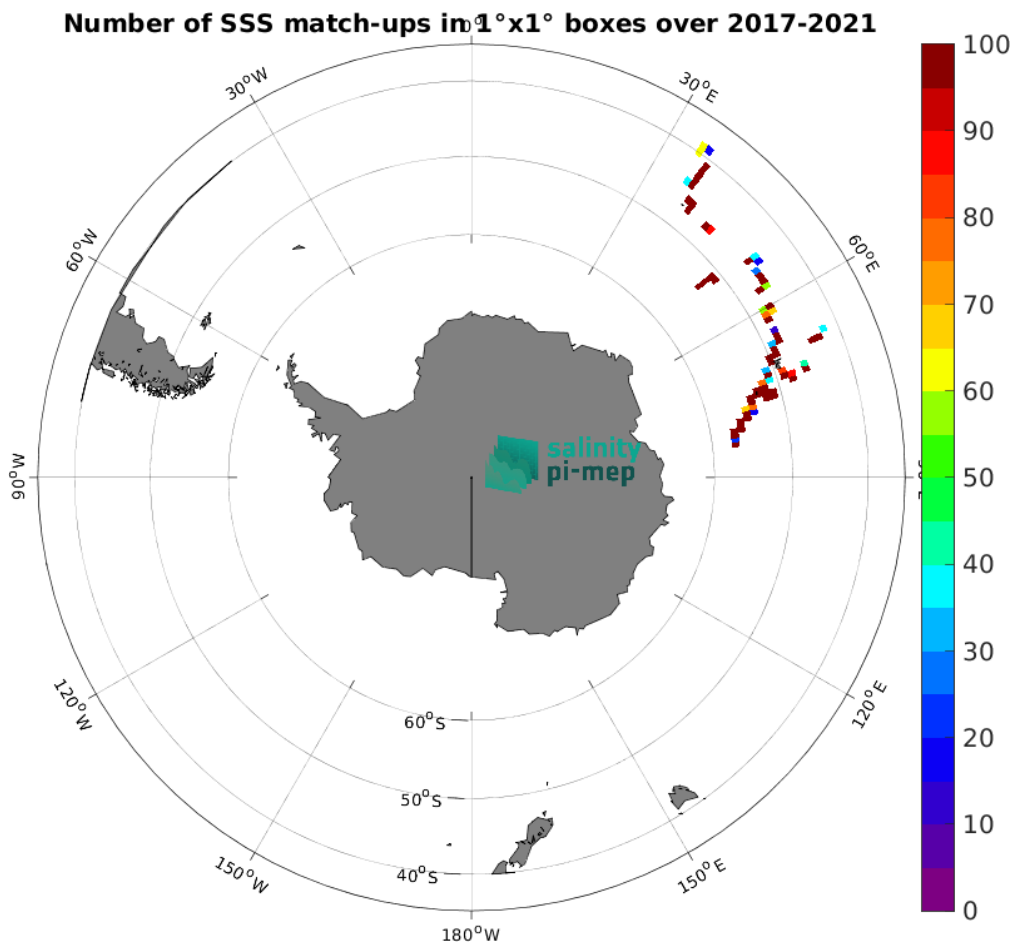
Figure 5: Number of SSS match-ups between TSG (GOSUD-Research-vessel) SSS and the SMAP SSS L2 v5.0 (JPL) SSS product for the Roaring Forties and Furious Fifties Pi-MEP region over 1^\circ \times 1^\circ boxes and for the full satellite product period.
