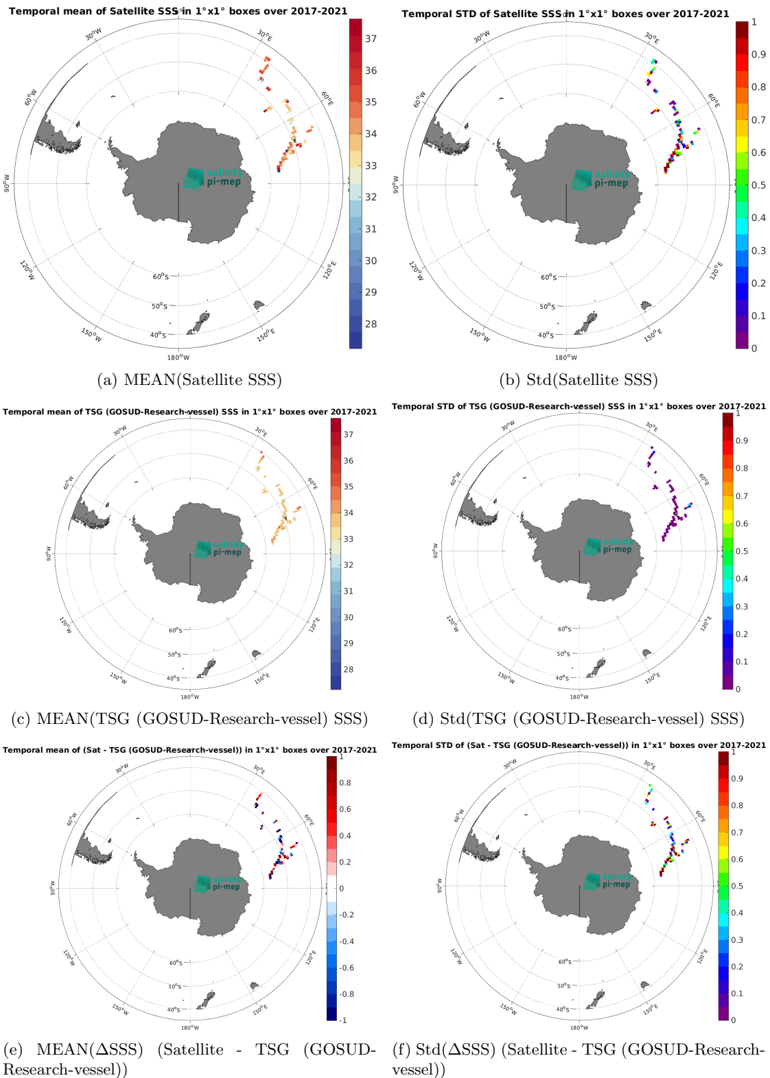
Figure 7: Temporal mean (left) and Std (right) of SSS from SMAP SSS L2 v5.0 (JPL) (top), TSG (GOSUD-Research-vessel) (middle), and of \Delta SSS (Satellite - TSG (GOSUD-Research-vessel)). Only match-up pairs are used to generate these maps.
