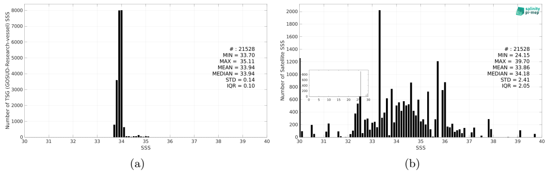
Figure 3: Histograms of SSS from TSG (GOSUD-Research-vessel) (a) and SMAP SSS L2 v5.0 (JPL) (b) considering all match-up pairs per bins of 0.1 over the Roaring Forties and Furious Fifties Pi-MEP region and for the full satellite product period.
