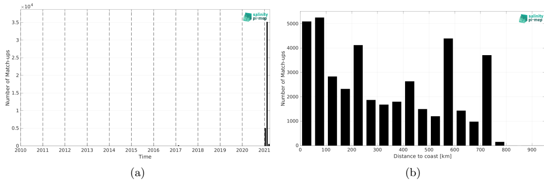
Figure 1: Number of match-ups between TSG (GOSUD-Research-vessel) and SMAP SSS L2 v5.0 (JPL) SSS as a function of time (a) and as function of the distance to coast (b) over the Roaring Forties and Furious Fifties Pi-MEP region and for the full satellite product period.
