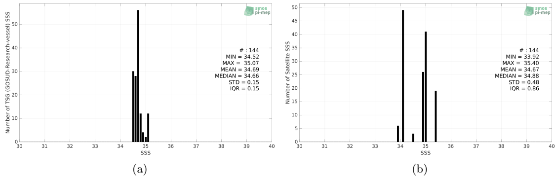
Figure 2: Histograms of SSS from TSG (GOSUD-Research-vessel) (a) and SMAP SSS L2 v5.0 (JPL) (b) considering all match-up pairs per bins of 0.1 over the Roaring Forties and Furious Fifties Pi-MEP region and for the full satellite product period.
