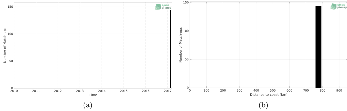
Figure 1: Number of match-ups between TSG (GOSUD-Research-vessel) and SMAP SSS L2 v5.0 (JPL) SSS as a function of time (a) and as function of the distance to coast (b) over the Roaring Forties and Furious Fifties Pi-MEP region and for the full satellite product period.
