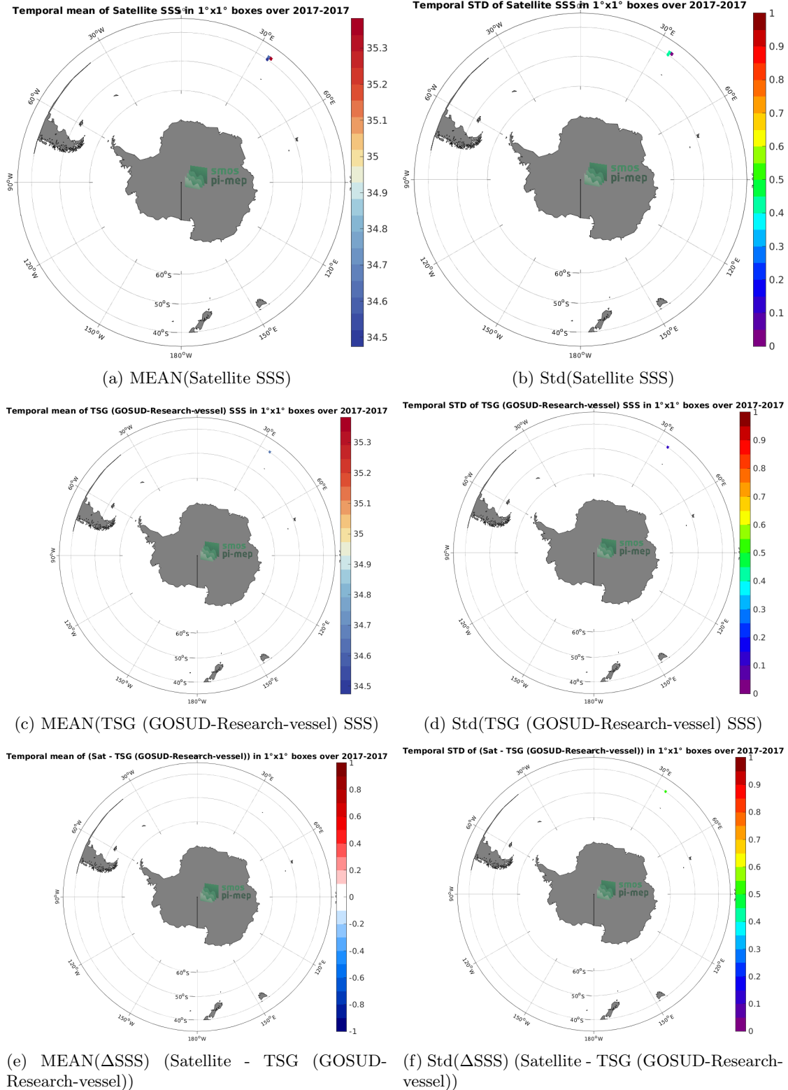
Figure 6: Temporal mean (left) and Std (right) of SSS from SMAP SSS L2 v5.0 (JPL) (top), TSG (GOSUD-Research-vessel) (middle), and of \Delta SSS (Satellite - TSG (GOSUD-Research-vessel)). Only match-up pairs are used to generate these maps.
