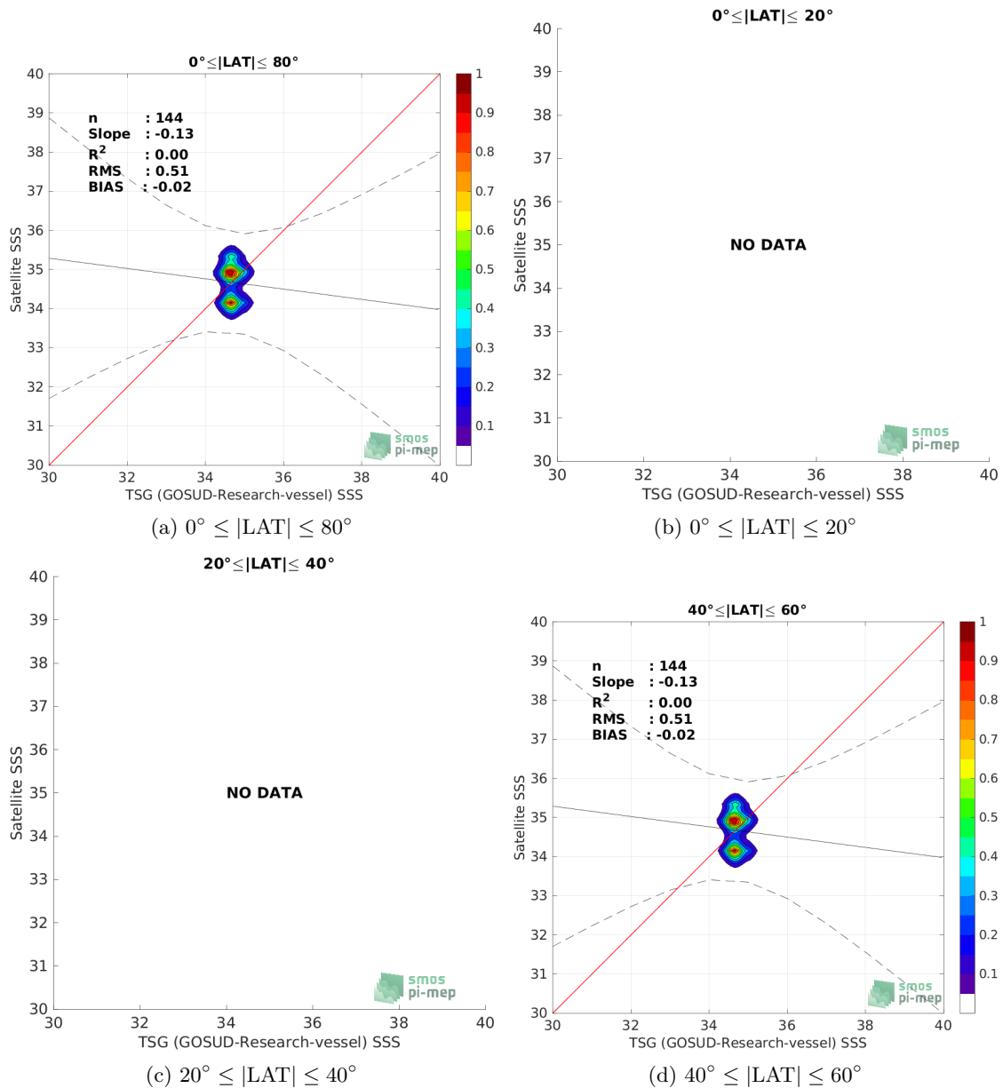
Figure 9: Contour maps of the concentration of SMAP SSS L2 v5.0 (JPL) SSS (y-axis) versus TSG (GOSUD-Research-vessel) SSS (x-axis) at match-up pairs for different latitude bands. For each plot, the red line shows x=y . The black thin and dashed lines indicate a linear fit through the data cloud and the \pm 95\% confidence levels, respectively. The number match-up pairs n , the slope and R^2 coefficient of the linear fit, the root mean square (RMS) and the mean bias between satellite and in situ data are indicated for each latitude band in each plot.
