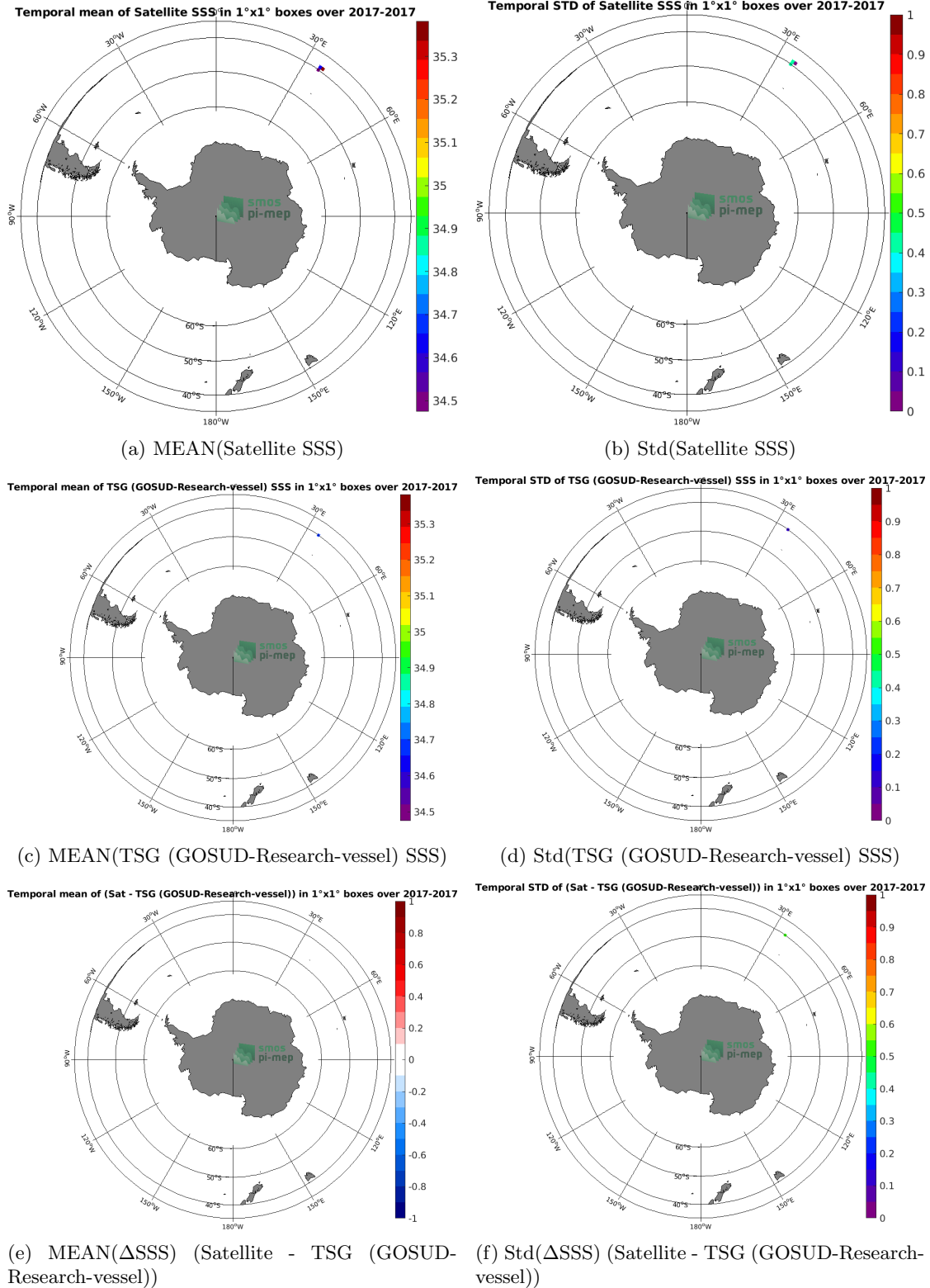
Figure 6: Temporal mean (left) and Std (right) of SSS from SMAP SSS L2 v5.0 (JPL) (top), TSG (GOSUD-Research-vessel) (middle), and of \Delta SSS (Satellite - TSG (GOSUD-Research-vessel)). Only match-up pairs are used to generate these maps.
