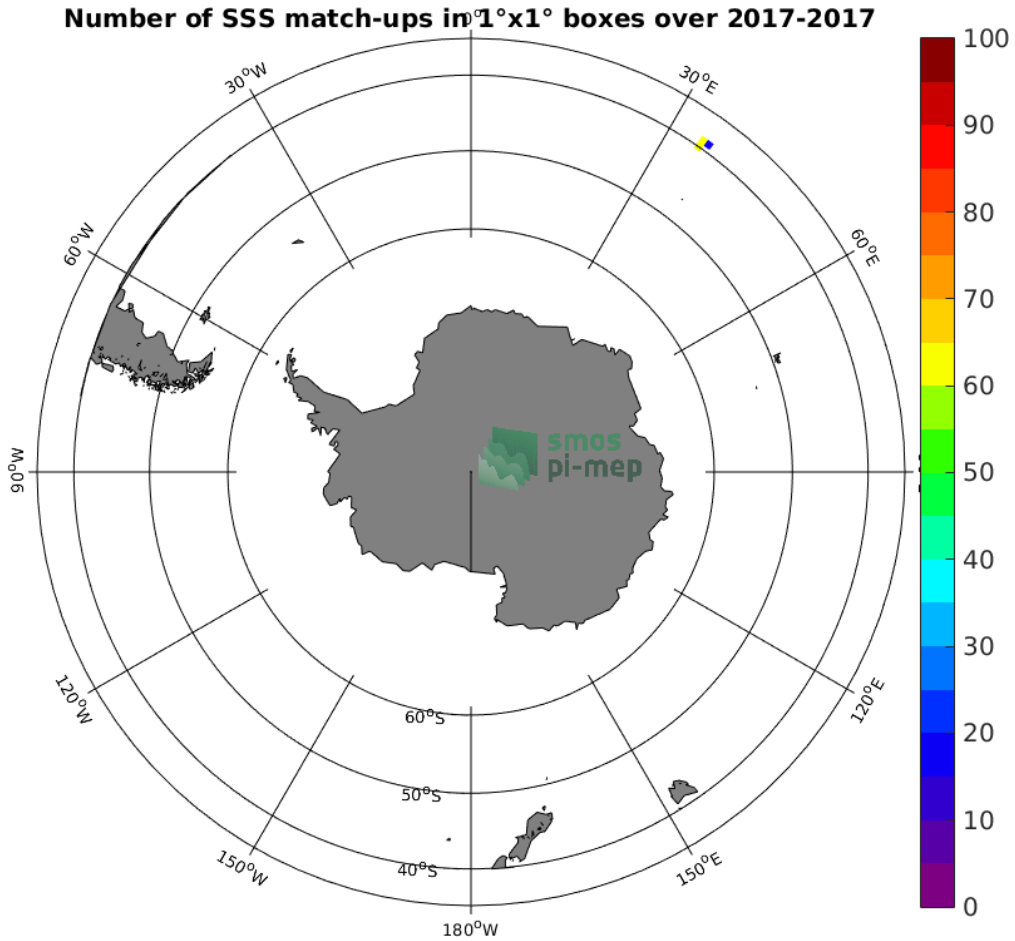
Figure 4: Number of SSS match-ups between TSG (GOSUD-Research-vessel) SSS and the SMAP SSS L2 v5.0 (JPL) SSS product for the Roaring Forties and Furious Fifties Pi-MEP region over 1°x1° boxes and for the full satellite product period.
