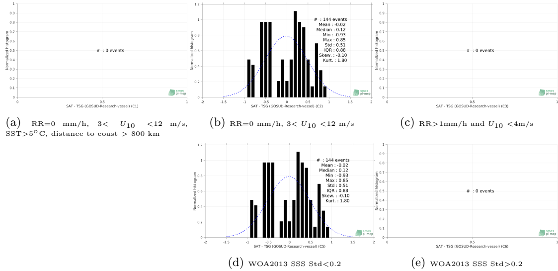
Figure 13: Normalized histogram of \Delta SSS (SMAP SSS L2 v5.0 (JPL) - TSG (GOSUD-Research-vessel)) for 5 different subdatasets corresponding to: RR=0 mm/h, 3 < U_{10} < 12 m/s, SST >5^{\circ} C, distance to coast > 800 km (a), RR=0 mm/h, 3 < U_{10} < 12 m/s (b), RR >1 mm/h and U_{10} < 4 m/s (c), WOA2013 SSS Std <0.2 (d), WOA2013 SSS Std >0.2 (e).
