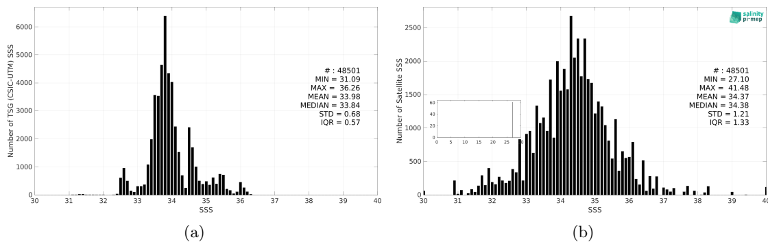
Figure 3: Histograms of SSS from TSG (CSIC-UTM) (a) and SMAP SSS L2 v5.0 (JPL) (b) considering all match-up pairs per bins of 0.1 over the Roaring Forties and Furious Fifties Pi-MEP region and for the full satellite product period.
