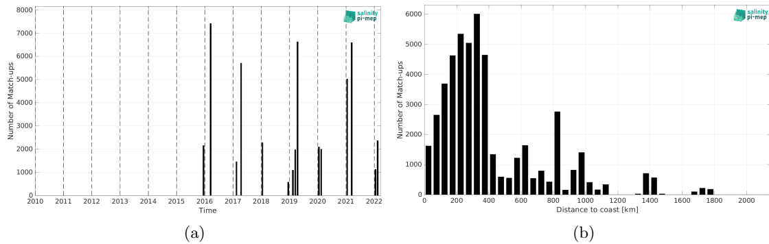
Figure 2: Number of match-ups between TSG (CSIC-UTM) and SMAP SSS L2 v5.0 (JPL) SSS as a function of time (a) and as function of the distance to coast (b) over the Roaring Forties and Furious Fifties Pi-MEP region and for the full satellite product period.
