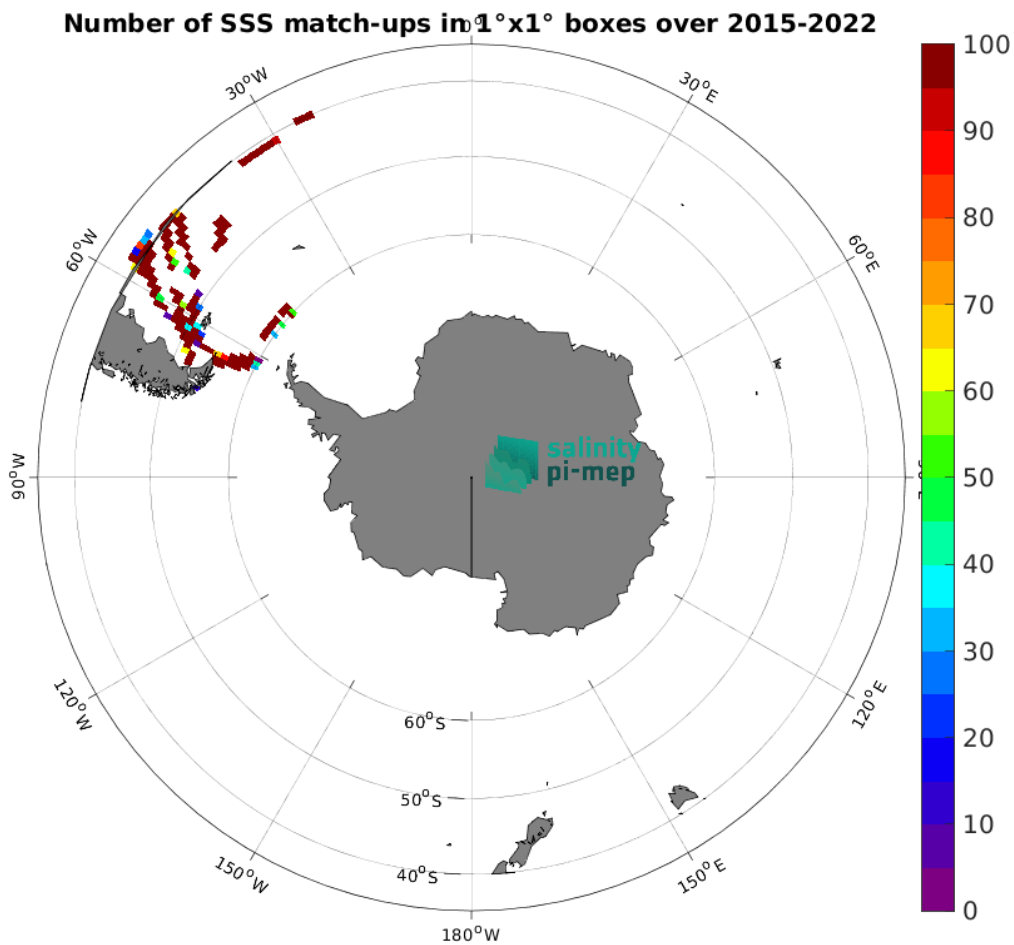
Figure 5: Number of SSS match-ups between TSG (CSIC-UTM) SSS and the SMAP SSS L2 v5.0 (JPL) SSS product for the Roaring Forties and Furious Fifties Pi-MEP region over 1^\circ \times 1^\circ boxes and for the full satellite product period.
