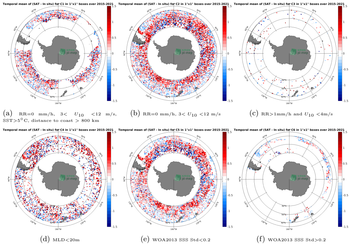
Figure 12: Temporal mean gridded over spatial boxes of size 1^{\circ}\times 1^{\circ} of \Delta\text{SSS} (SMAP SSS L2 v5.0 (JPL) - Argo) for 6 different subdatasets corresponding to: \text{RR}=0 mm/h, 3 < U_{10} < 12 m/s, \text{SST}>5^{\circ}\text{C} , distance to coast > 800 km (a), \text{RR}=0 mm/h, 3 < U_{10} < 12 m/s (b), \text{RR}>1 mm/h and U_{10} < 4 m/s (c), \text{MLD}<20\text{m} (d), \text{WOA2013 SSS Std}<0.2 (e), \text{WOA2013 SSS Std}>0.2 (f).
