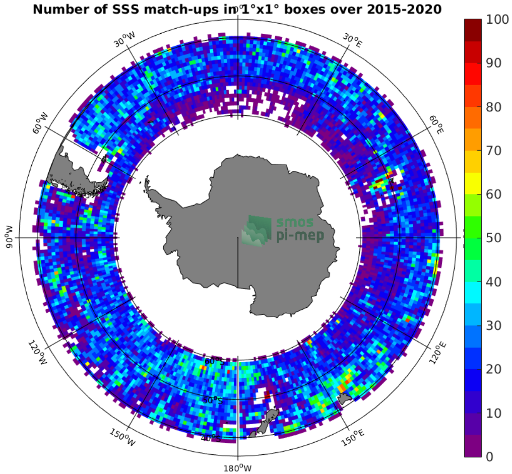
Figure 4: Number of SSS match-ups between Argo SSS and the SMAP SSS L2 v5.0 (JPL) SSS product for the Roaring Forties and Furious Fifties Pi-MEP region over 1°x1° boxes and for the full satellite product period.
