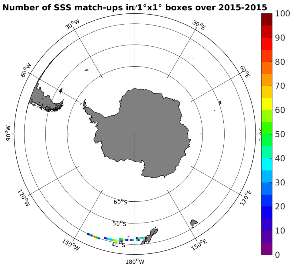
Figure 4: Number of SSS match-ups between TSG-LEGOS-DM SSS and the SMAP-L2-JPL-V4 SSS product for the Roaring Forties and Furious Fifties Pi-MEP region over 1^\circ \times 1^\circ boxes and for the full satellite product period.
