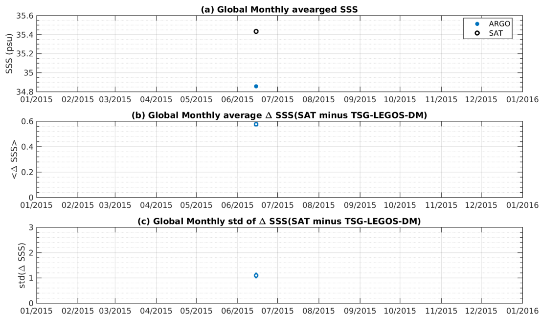
Figure 7: Time series of the monthly averaged mean SSS (top), mean \Delta SSS (Satellite - TSG-LEGOS-DM) and STD of \Delta SSS (Satellite - TSG-LEGOS-DM) over the Roaring Forties and Furious Fifties Pi-MEP region considering all match-ups collected by the Pi-MEP platform.
