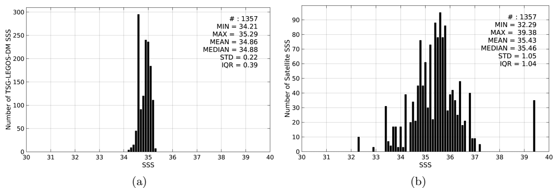
Figure 2: Histograms of SSS from TSG-LEGOS-DM (a) and SMAP-L2-JPL-V4 (b) considering all match-up pairs per bins of 0.1 over the Roaring Forties and Furious Fifties Pi-MEP region and for the full satellite product period.
