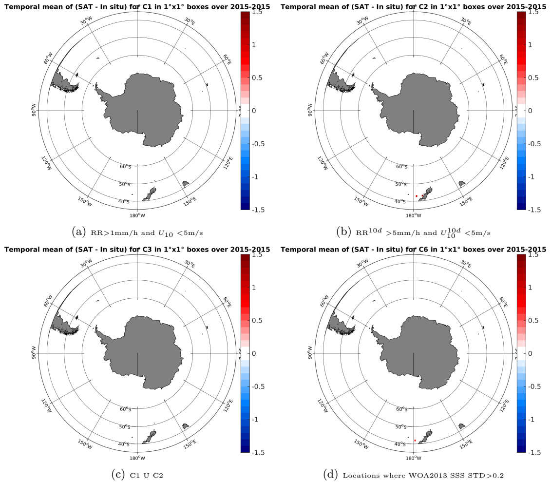
Figure 12: Temporal mean gridded over spatial boxes of size 1°x1° of \Delta SSS (SMAP-L2-JPL-V4 - TSG-LEGOS-DM) for 4 different subdatasets corresponding to: RR > 1\text{mm/h} and U_{10} < 5\text{m/s} (a), RR^{10d} > 5\text{mm/h} and U_{10}^{10d} < 5\text{m/s} (b), C1 U C2 (c), Locations where WOA2013 SSS STD > 0.2 (d).
