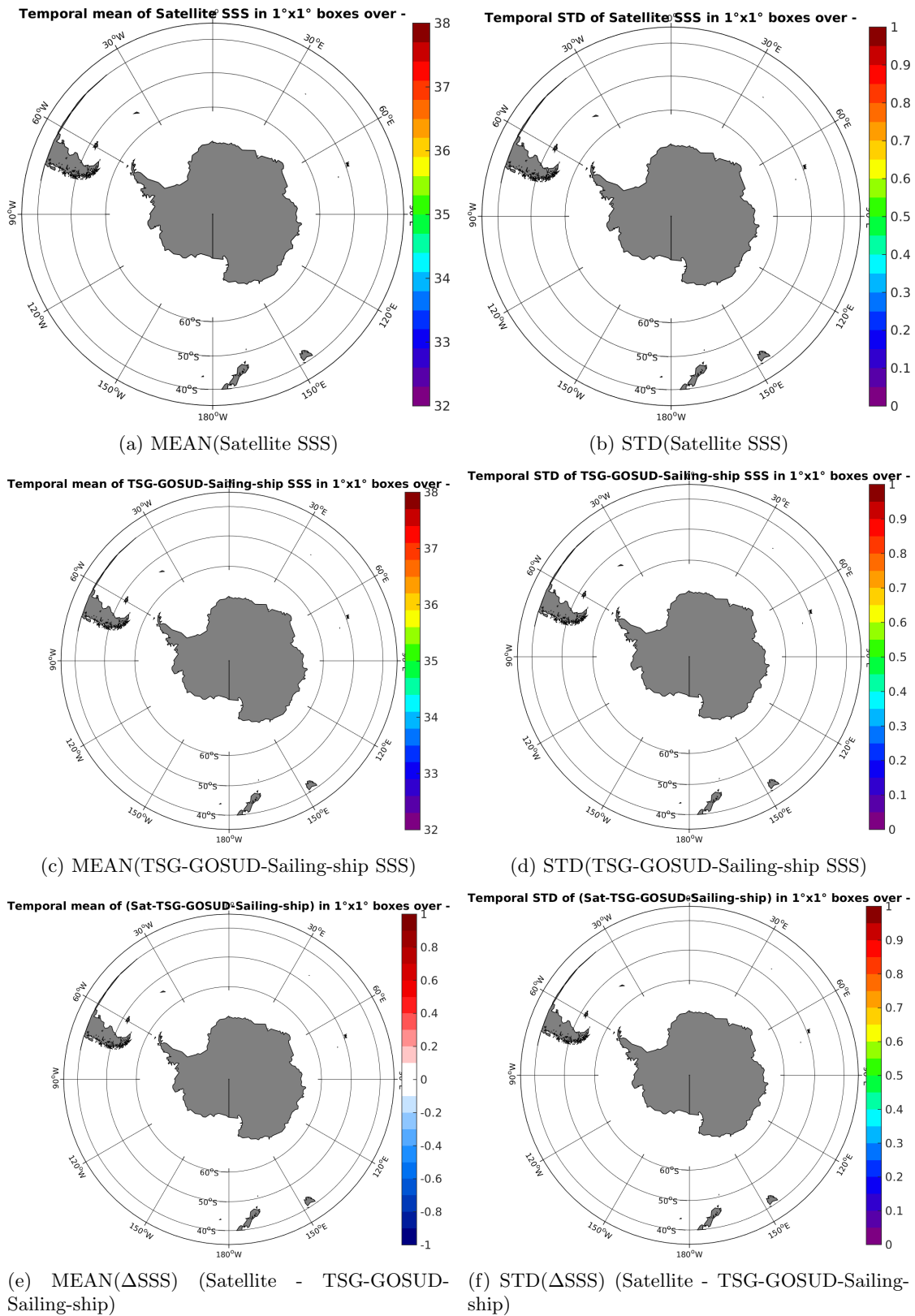
Figure 6: Temporal mean (left) and STD (right) of SSS from SMAP-L2-JPL-V4 (top), TSG-GOSUD-Sailing-ship (middle), and of \Delta SSS (Satellite - TSG-GOSUD-Sailing-ship). Only match-up pairs are used to generate these maps.
