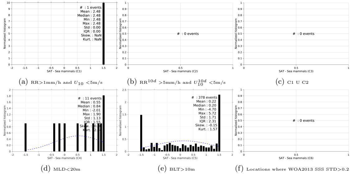
Figure 13: Normalized histogram of \Delta SSS (SMAP-L2-JPL-V4 - Sea mammals) for 6 different sub-datasets corresponding to: RR > 1mm/h and U_{10} < 5 m/s (a), RR^{10d} > 5 mm/h and U_{10}^{10d} < 5 m/s (b), C1 U C2 (c), MLD < 20m (d), BLT > 10m (e), Locations where WOA2013 SSS STD > 0.2 (f).
