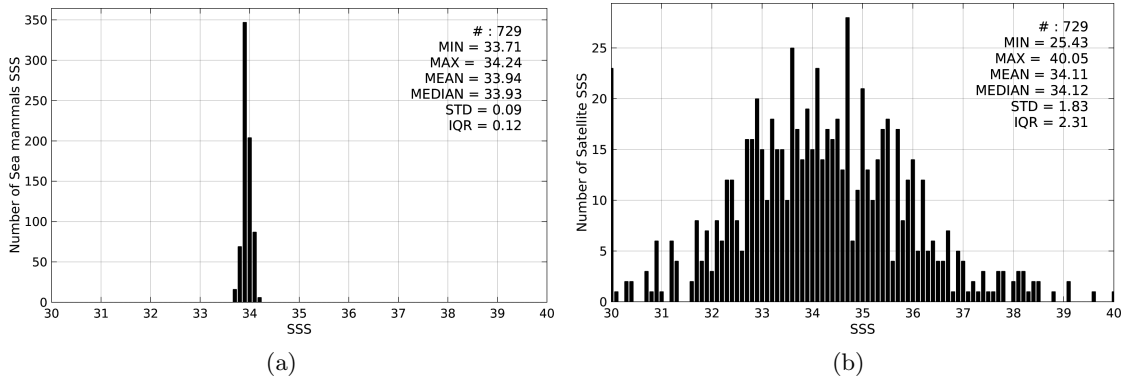
Figure 2: Histograms of SSS from Sea mammals (a) and SMAP-L2-JPL-V4 (b) considering all match-up pairs per bins of 0.1 over the Roaring Forties and Furious Fifties Pi-MEP region and for the full satellite product period.
