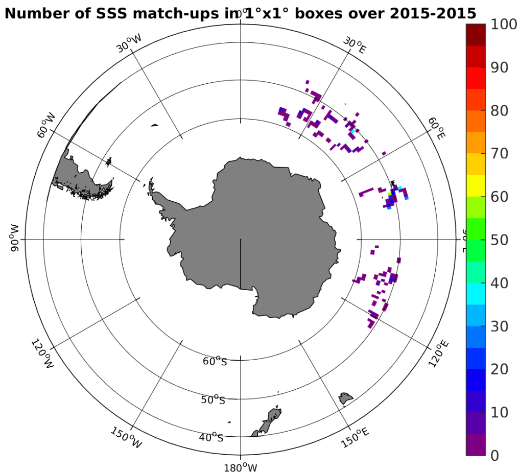
Figure 4: Number of SSS match-ups between Sea mammals SSS and the SMAP-L2-JPL-V4 SSS product for the Roaring Forties and Furious Fifties Pi-MEP region over 1°x1° boxes and for the full satellite product period.
