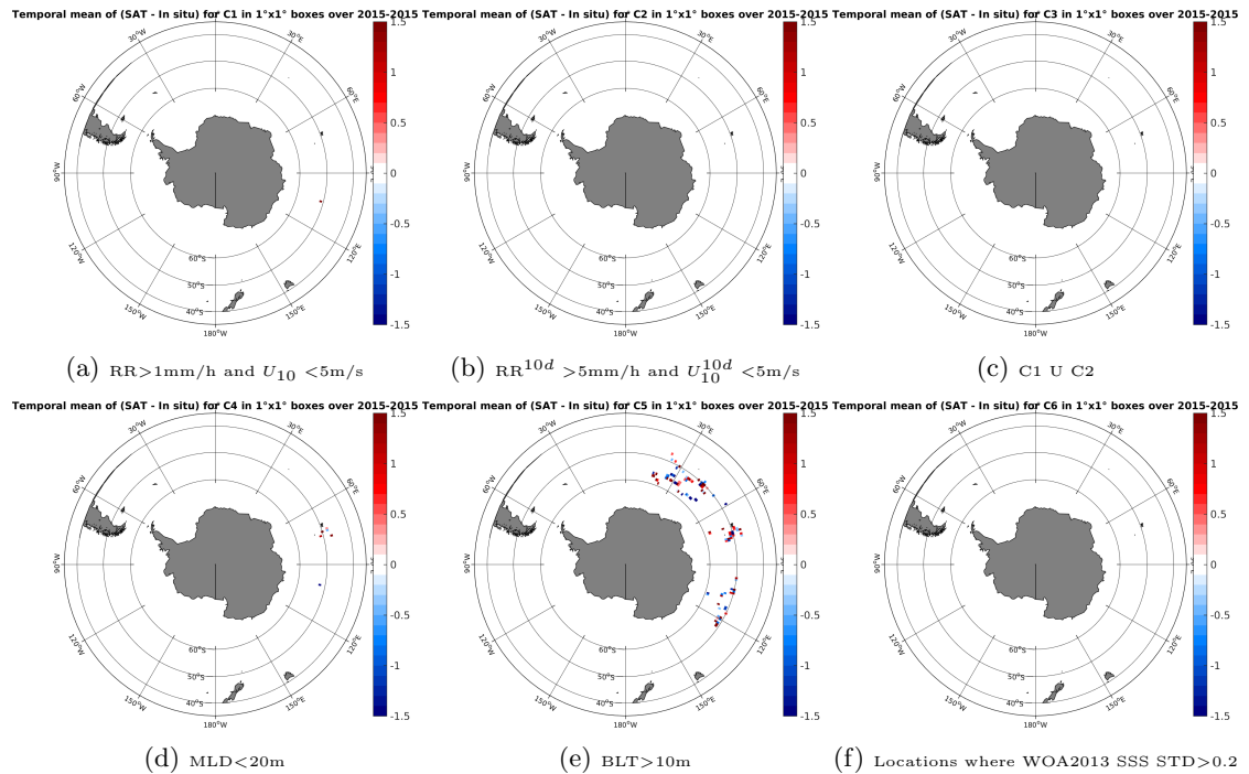
Figure 12: Temporal mean gridded over spatial boxes of size 1^\circ \times 1^\circ of \Delta SSS (SMAP-L2-JPL-V4 - Sea mammals) for 6 different subdatasets corresponding to: RR > 1\text{mm/h} and U_{10} < 5\text{m/s} (a), RR^{10d} > 5\text{mm/h} and U_{10}^{10d} < 5\text{m/s} (b), C1 U C2 (c), MLD < 20\text{m} (d), BLT > 10\text{m} (e), Locations where WOA2013 SSS STD > 0.2 (f).
